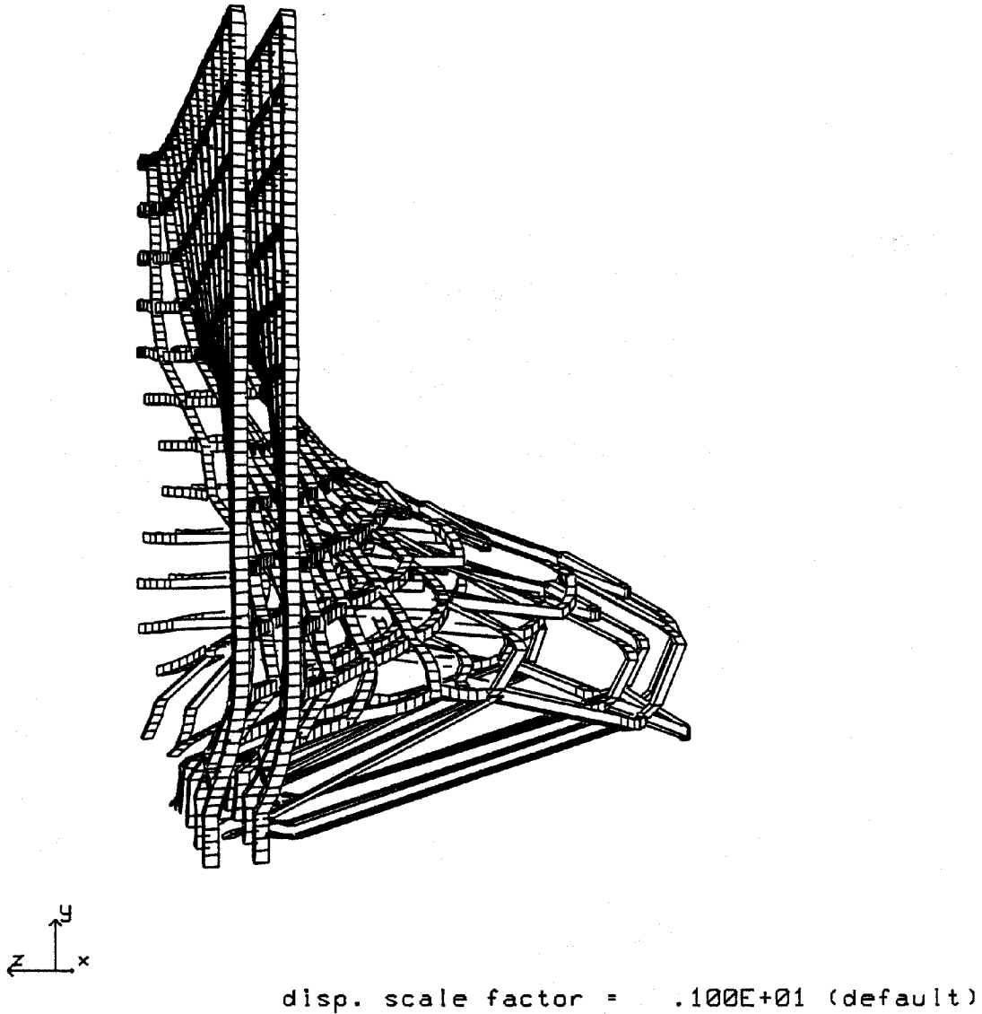
Figure 6 - Deformation of steel reinforcing bars at approximately 0.025 second after loading.
