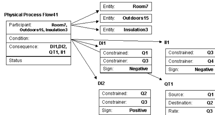
Figure 4.8: Process frame – Example 2
