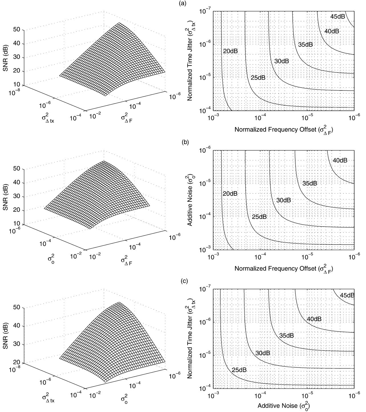
Fig. 5. Signal to noise and distortion ratio for frequency domain ADC with N = 5 . No gain distortion is included (i.e., E\{g_n^2\} = 1 ). (a-left column) Normalized timing errors second moment ( \sigma_{\Delta tx}^2 ) versus normalized frequency offset second moment ( \sigma_{\Delta F}^2 ) for \sigma_o^2 = 10^{-6} , and in (a-right column) isolines. (b-left column) Additive noise second moment ( \sigma_o^2 ) versus normalized frequency offset second moment ( \sigma_{\Delta F}^2 ) for \sigma_{\Delta tx}^2 = 10^{-6} , and in (a-right column) isolines. (c-left column) Normalized timing errors second moment ( \sigma_{\Delta tx}^2 ) versus additive noise second moment ( \sigma_o^2 ) for \sigma_{\Delta F}^2 = 10^{-6} , and in (c-right column) isolines.
