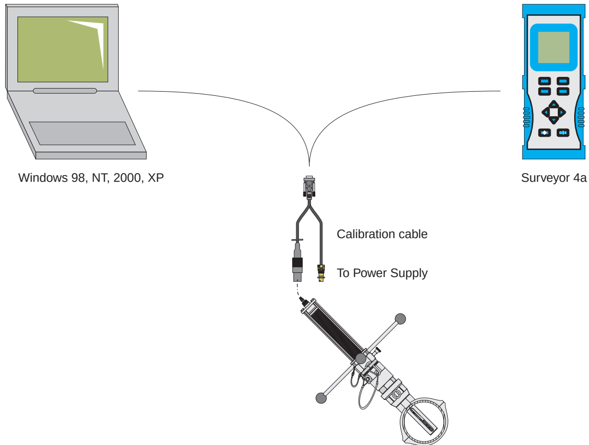
Figure 22 Operations Setup
