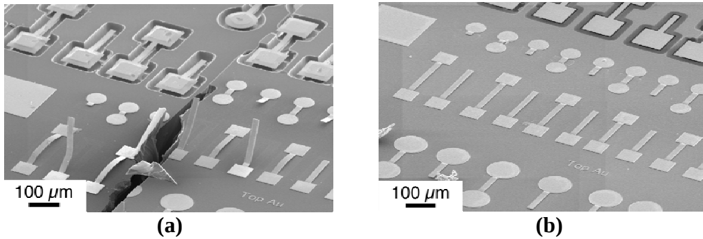
Figure 11: Fixed-fixed and cantilever beams made of the Top Au layer after loading at (a) 1 \times 10^9 g, and (b) 2 \times 10^9 g.
