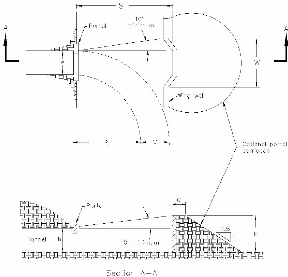
Figure C5.F4. Portal Barricade Location, Height and Width (see paragraph C5.3.4.)
