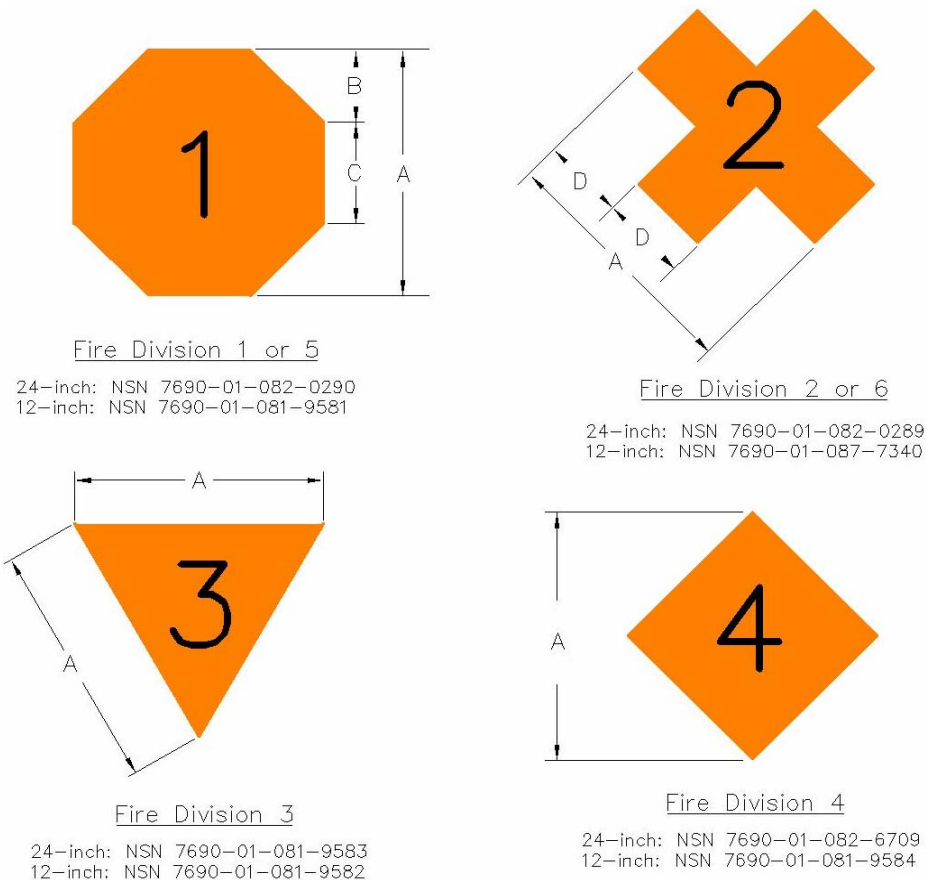
Figure C8.F1. Fire Division Symbols
