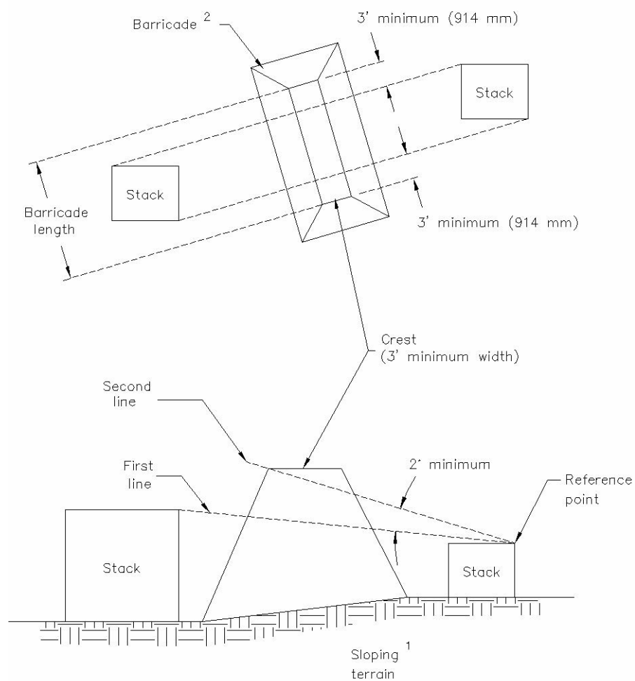
Figure C5.F3. Determination of Barricade Length and Height (see subparagraph C5.3.2.3.)
