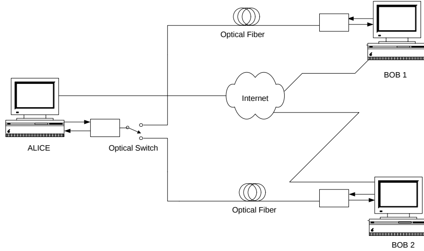
Figure 1. Schematic diagram of a QKD network with one Alice and two Bobs
