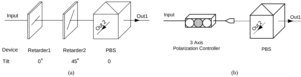
Figure 3. Two kinds of PRAC setting: Liquid Crystal Retardance (a) and Piezo Polarization Controllers (b)
