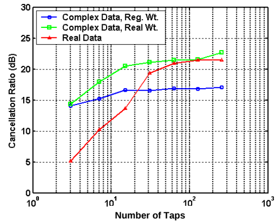
Fig. 5. Cancellation performance of the pre-filtered data in the 2 nd experimental test for a TFC vs. number of taps: complex data using complex and real weights, and real data using real weights
