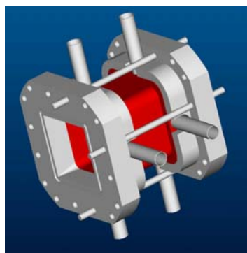
Fig.2 – Cooled composite combustion chamber duct (in red) tested at ONERA ATD5
