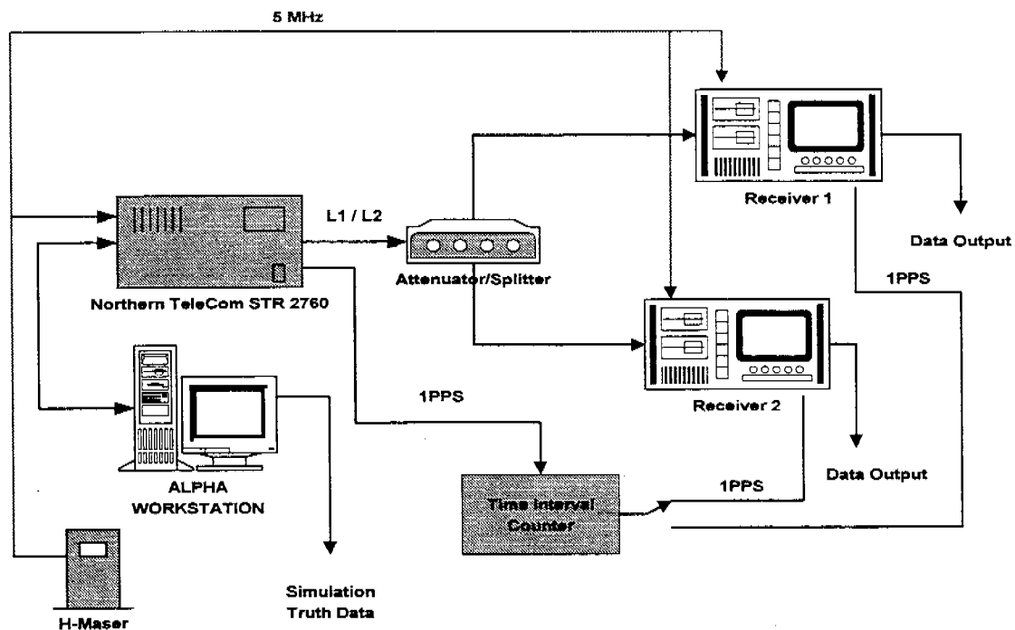
Figure 1. Simulation Configuration
