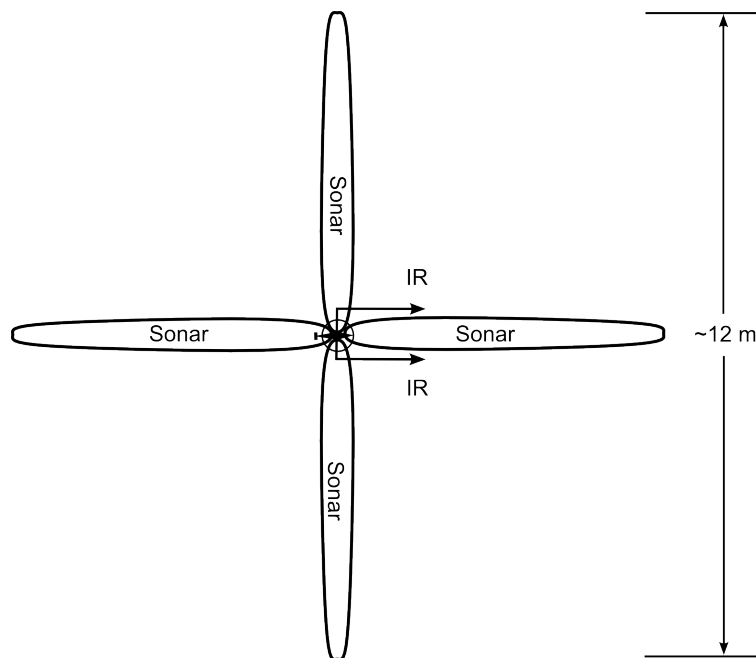
Figure 17: Range sensor layout.
