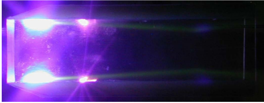
Figure 132. Discharge along Inlet Sidewalls, E=650V , I=40\text{ mA}
