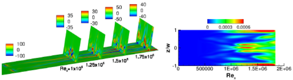
Figure 232. \Delta T_w = 2.52 T_{ad} (Case 8)
