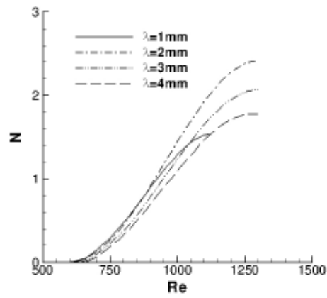
Figure 210. Spanwise Wavelength
