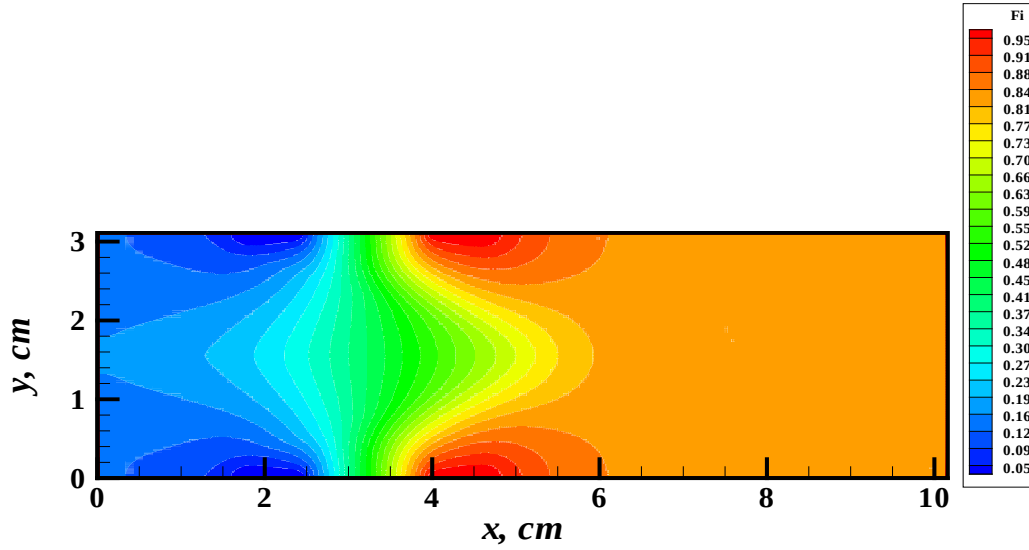
Figure 61. Electric Potential Distribution; E=500 volt, T_w = 300 K and \eta = 0.1
