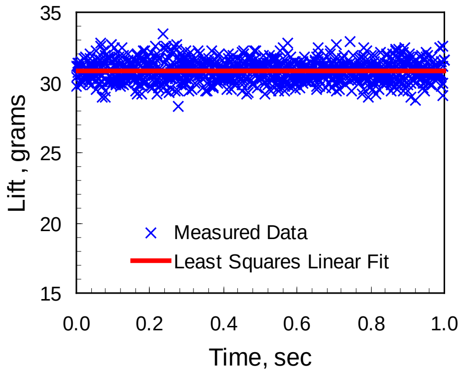
Figure 94. Lift Measurements as a Function of Time for 0° Angle Of Attack
