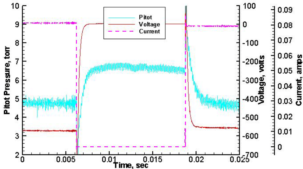
Figure 84. Averaged Pitot Probe Measurements in a Mach 5 Flow with an 80 mA Discharge that is Oscillated at 40 Hz
