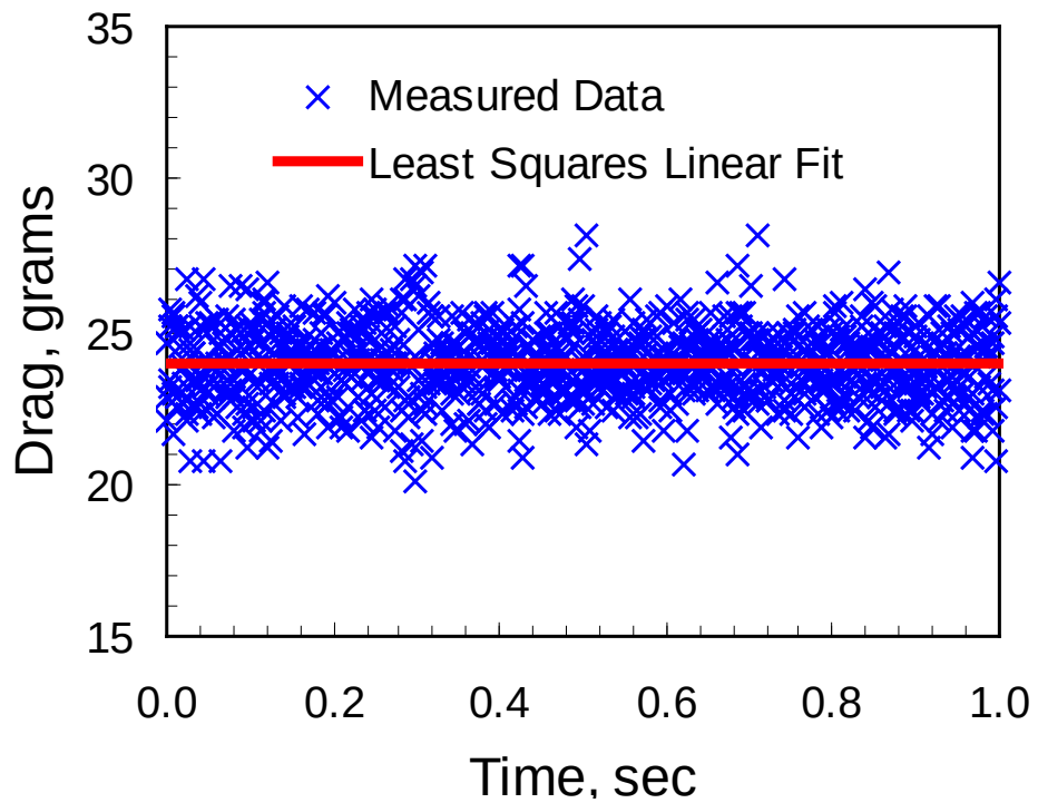
Figure 95. Drag Measurements as a Function of Time for 0° Angle Of Attack
