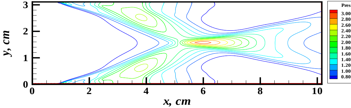
Figure 65. Pressure Contours in Torr; E = 500 volt and T_w = 300 K
