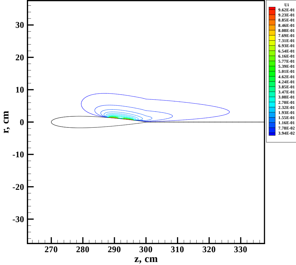
Figure 14. Concentration of Charge Particles, 10^{10} \text{ cm}^{-3} , for NACA-0012 at M=2 and Re = 1000 , \alpha = 10^\circ , and E=700 V
