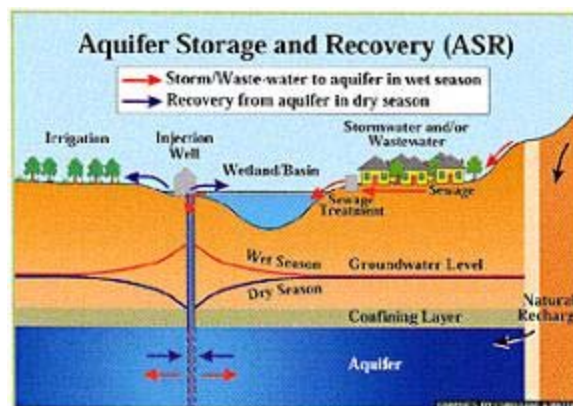
Figure D3. Aquifer storage and recovery.
