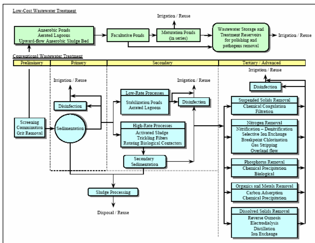
Figure D1. Wastewater reuse path.
