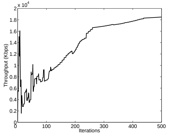
Figure 6: System Throughput Using a Perfect Reception Interference Threshold K
