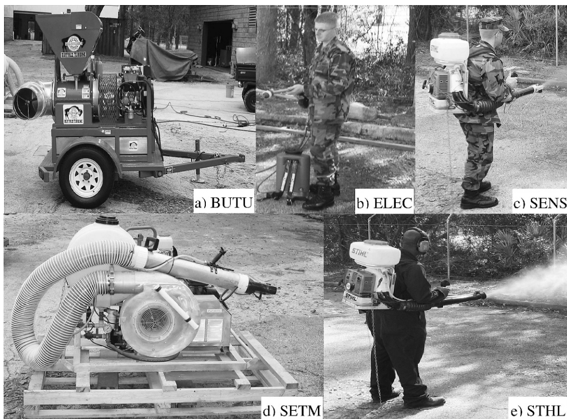
Fig. 2. Sprayers used in the study. a. BUTU, Buffalo Turbine; b. ELEC, Electroлон; c. SENS, Spectrum Electrostatic Nozzle on Stihl; d. SETM, Spectrum Electrostatic Truck Mounted; e. STHL, Stihl.
