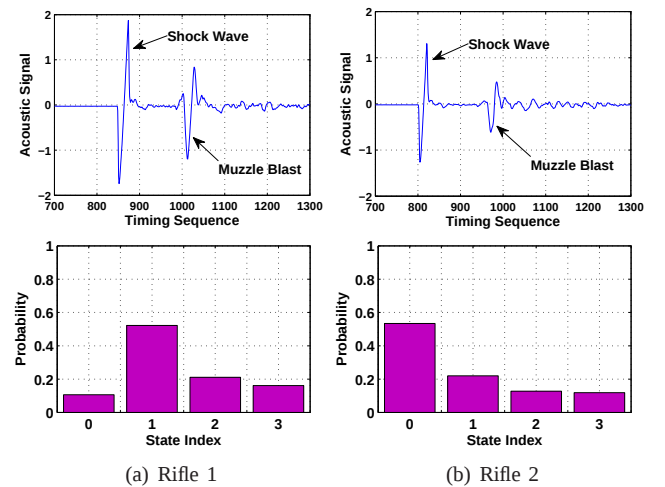
Fig. 4. Acoustic signals and respective feature vectors
