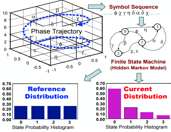
Fig. 1. Concept of Symbolic Dynamic Filtering (SDF)
