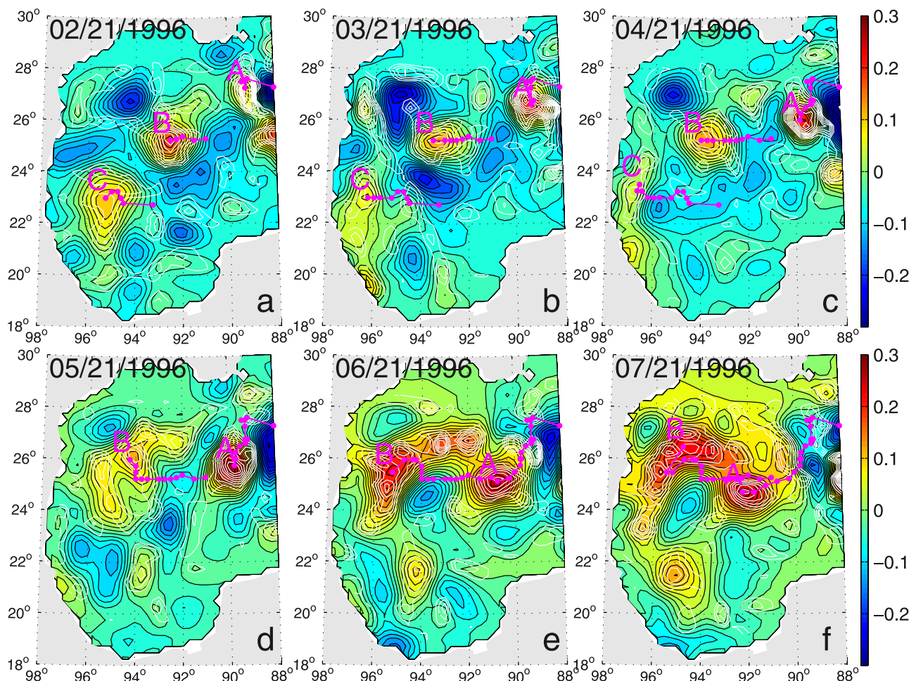
Figure 4. Sea level anomaly (color scale in m) in the western Gulf of Mexico for the period of February–July 1996 superimposed by Okubo-Weiss parameter (W, white contour). Only negative values of W are depicted with the interval of 2 \times 10^{-6} \text{ s}^{-2} . Trajectory of three major anticyclonic eddies (96A, 96B, and 96C) is depicted every 10 days (white dots) starting at 1 January 1996.
