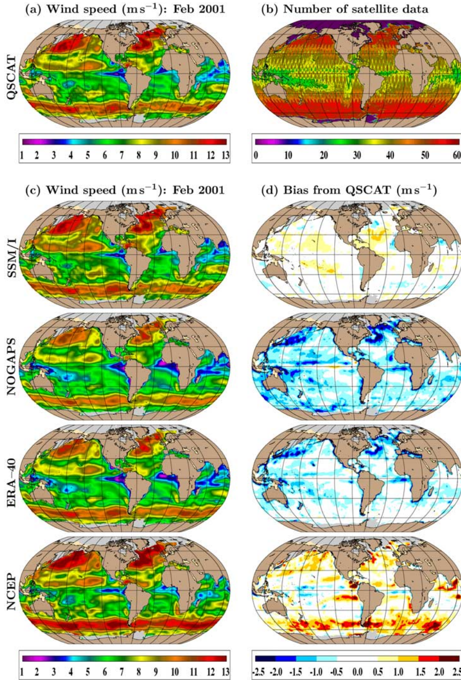
Figure 2. (a) Monthly mean rain-free winds at 10 m from QSCAT over the ice-free regions in February 2001; (b) number of rain-free wind observations used for forming winds in Figure 2a; (c) mean wind speeds from SSM/I, NOGAPS, ERA-40, and NCEP from top to bottom; and (d) difference in mean wind speed with respect to QSCAT for all products in Figure 2c, i.e., SSM/I-QSCAT, NOGAPS-QSCAT, etc. All are gridded to a resolution of 0.25^\circ \times 0.25^\circ .
