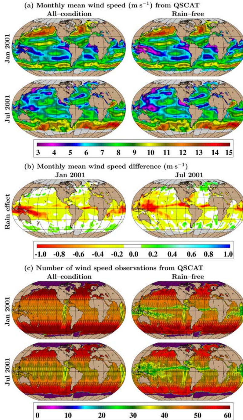
Figure 1. (a) 0.25^\circ \times 0.25^\circ resolution 10 m winds constructed from the QSCAT in January and July of 2001 when using (left) all-condition winds (rain-contaminated and rain-free) and (right) rain-free winds. (b) Differences in Figure 1a when subtracting the all-condition winds from the rain-free winds. Negative difference values in the color palette are shown in red. (c) Number of wind measurements used for forming monthly mean winds in Figure 1a for each month.
