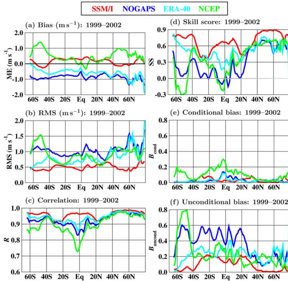
Figure 5. Zonal averages of statistical metrics shown in Figures 3 and 4. Zonal averages for conditional and unconditional biases used for calculating nondimensional skill score are also given. Zonal averaging was performed at each 0.25^\circ latitude belt.
