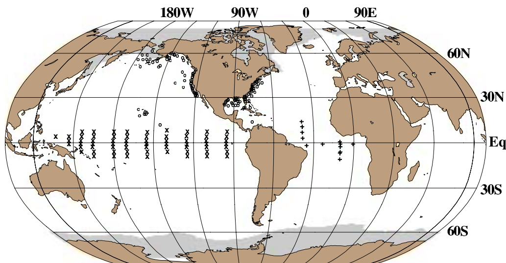
Figure 6. Locations of TAO (x), PIRATA (+) and NDBC (o) used in the analyses in this paper.
