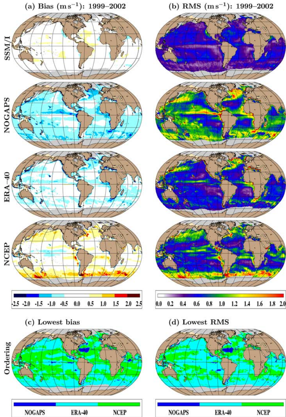
Figure 3. Spatial maps of mean (a) bias and (b) RMS difference in wind speed between QSCAT and other products from September 1999 through August 2002. The bias in Figure 3a was computed by subtracting QSCAT from other products, SSM/I-QSCAT, NOGAPS-QSCAT, etc. Also shown are NWP products giving (c) lowest bias and (d) lowest RMS with respect to QSCAT winds.
