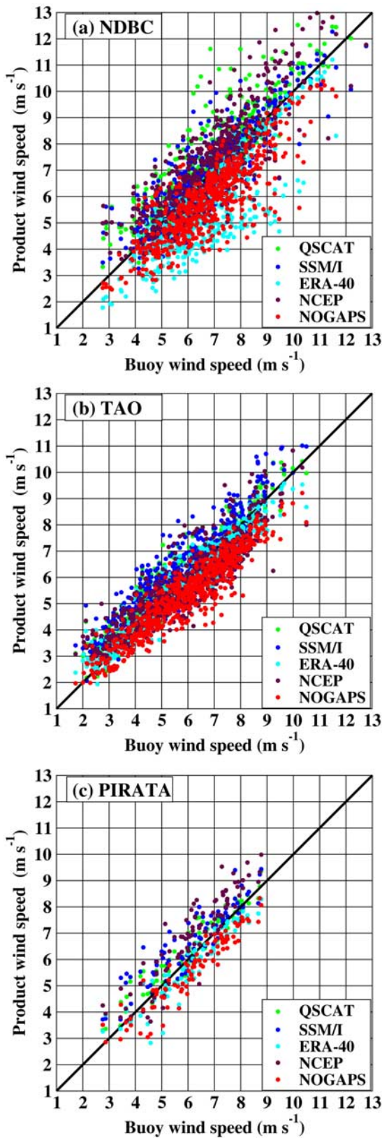
Figure 7. Scatterplots of monthly mean wind speeds at 10 m above the sea surface obtained from buoys versus those from various products. Results are shown at (a) NDBC, (b) TAO, and (c) PIRATA buoys in 2001.
