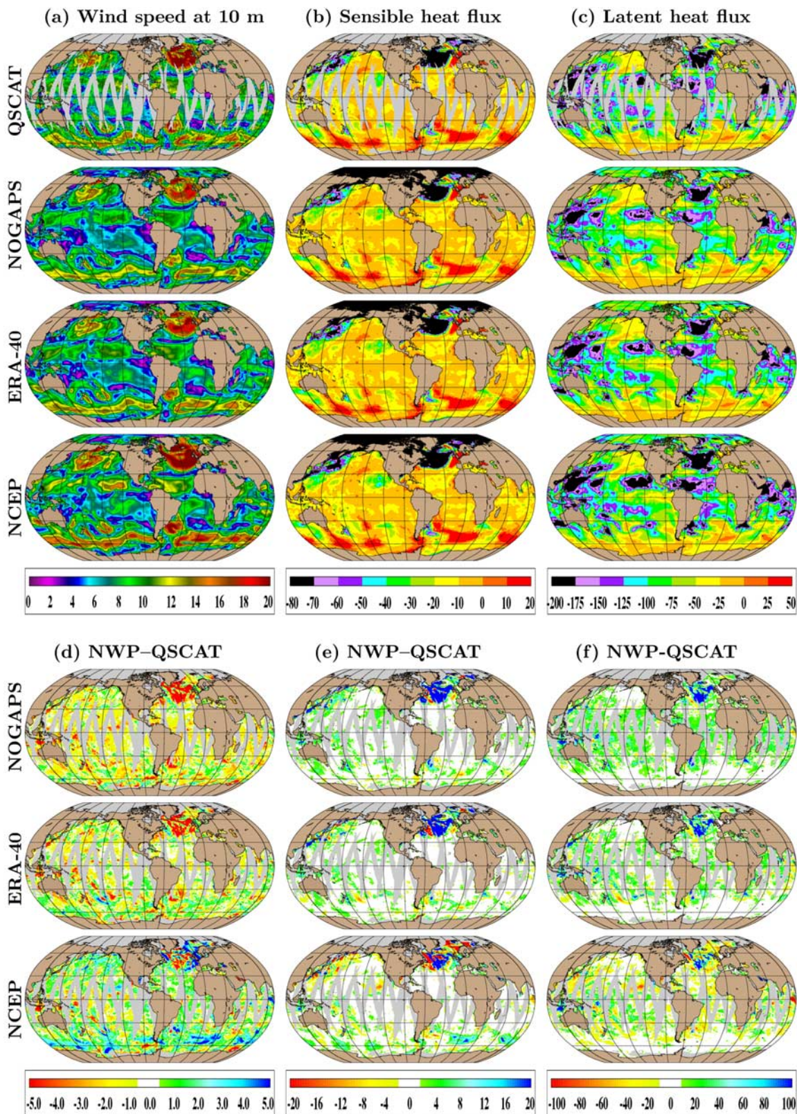
Figure 8. Spatial variations of the variables from QSCAT and NWP products on 1 February 2002: (a) wind speed ( \text{m s}^{-1} ), (b) sensible heat flux ( \text{W m}^{-2} ), and (c) latent heat flux ( \text{W m}^{-2} ). (d, e, and f) Differences for NWP products with respect to QSCAT.
