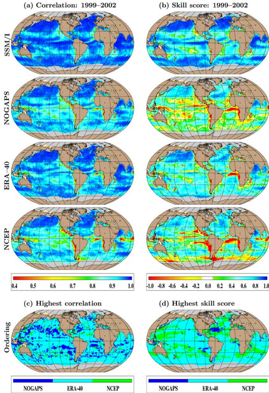
Figure 4. The same as Figure 3 but for (a) correlation coefficient and (b) nondimensional skill score. (c and d) NWP products giving highest correlation and highest skill in comparison to QSCAT winds. Negative skill values (red color tones) indicate poor agreement.
