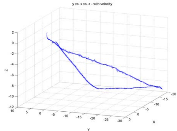
Fig. 3 – Sample 3-D Matlab plot of sample trial. Includes true heading, pitch, roll, depth and velocity information at 80Hz rate (velocity and depth at 20Hz rate).
