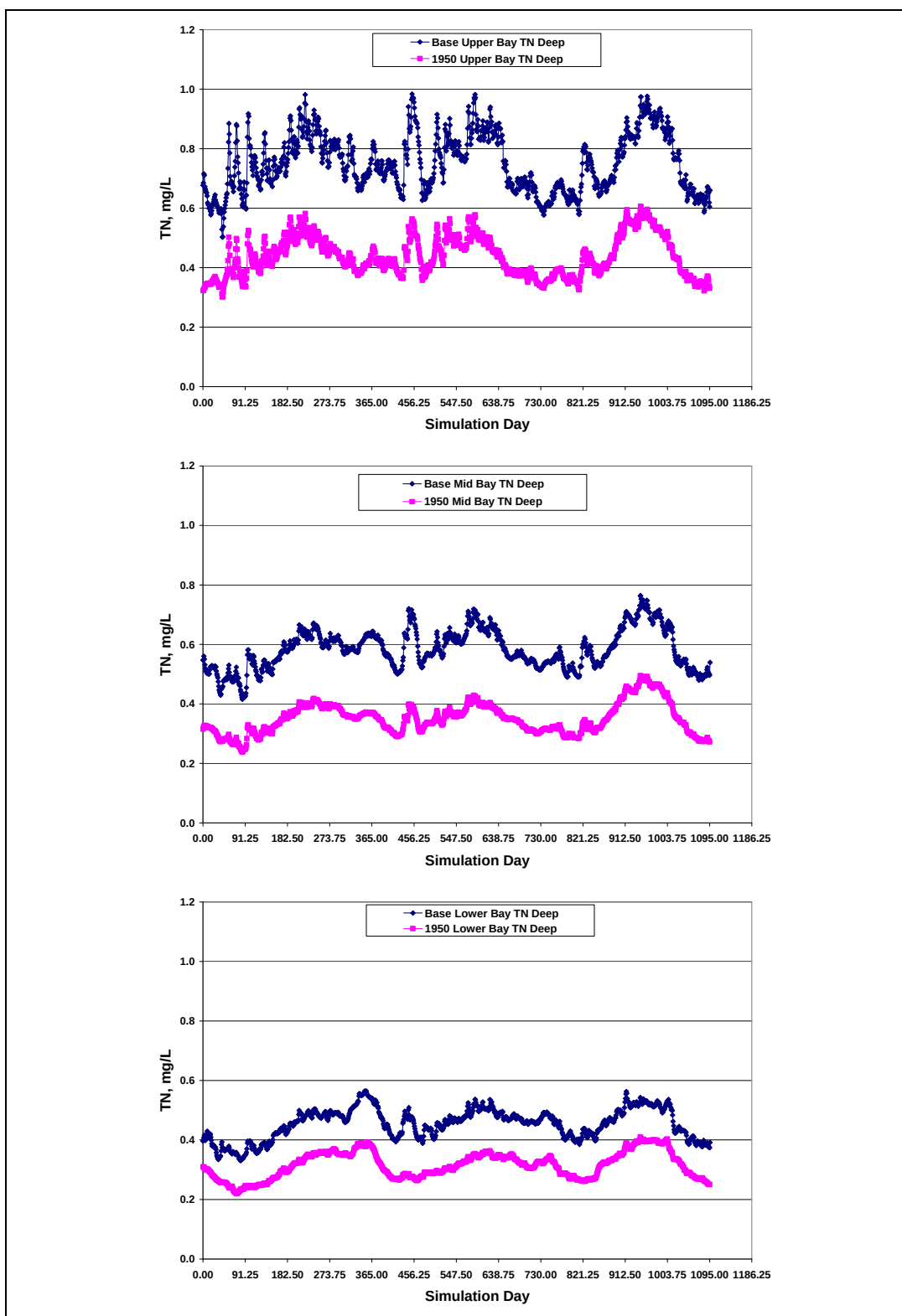
Figure 21. Comparison of the deep TN for base and 1950's RMB2 results in the upper, mid, and lower regions of the Chesapeake Bay.
