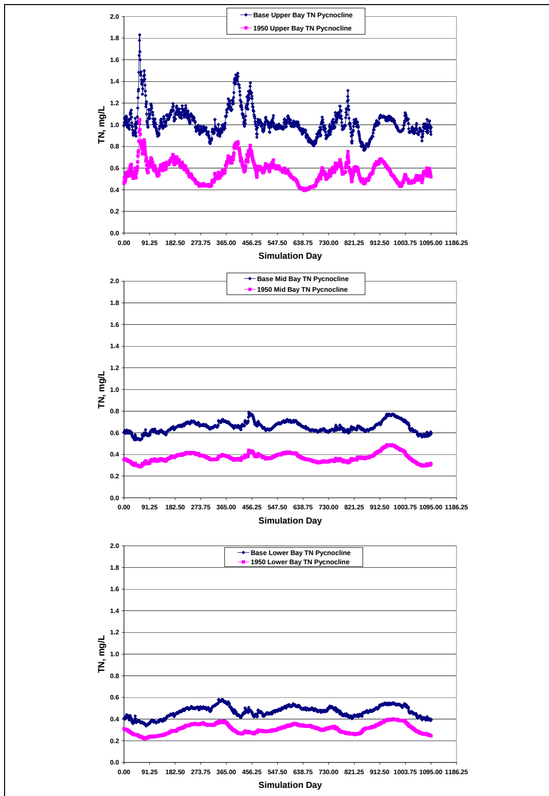
Figure 17. Comparison of the pycnocline TN for base and 1950's RMB2 results in the upper, mid, and lower regions of the Chesapeake Bay.
