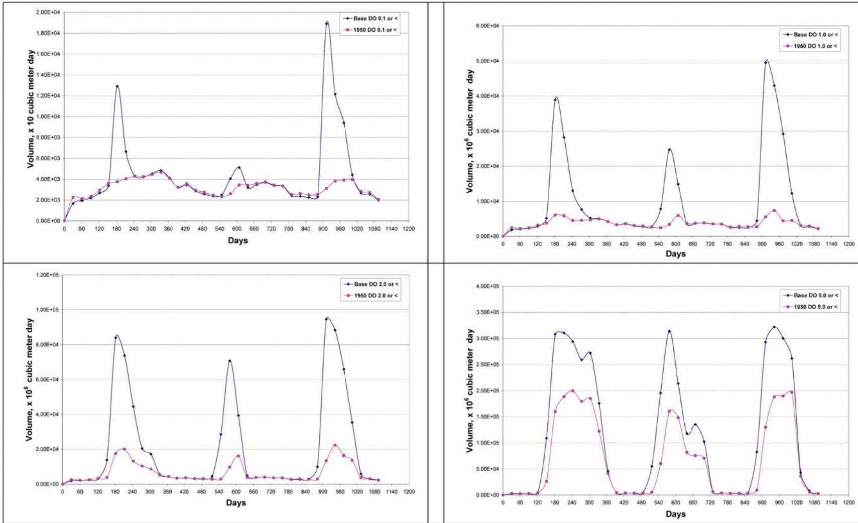
Figure 32. DO volume day for mid Chesapeake Bay region DO \leq 0.1 , 1.0, 2.0, and 5.0.
