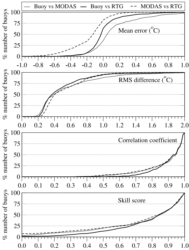
Figure 14. The percentage cumulative frequencies of statistical metrics shown in Figure 12. Median value corresponds to 50% in each panel.
