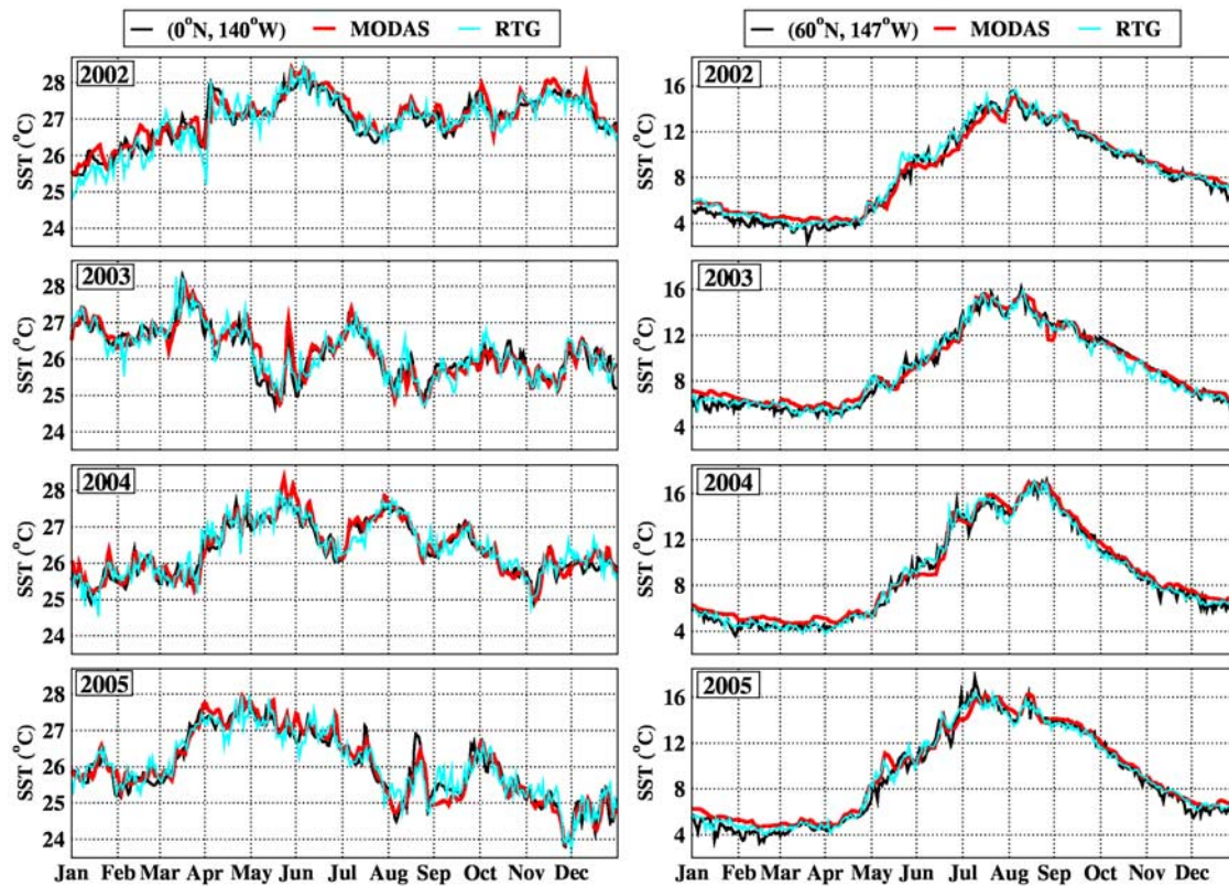
Figure 7. Daily SST time series from a TAO buoy at ( 0^{\circ}\text{N} , 140^{\circ}\text{W} ) and NDBC buoy at ( 60^{\circ}\text{N} , 147^{\circ}\text{W} ) (black) and those from MODAS (red) and RTG (cyan) as well in each year during 2002–2005. Any missing buoy SSTs are filled using linear interpolation. In all plots, the x-axis is labeled starting from the beginning of each month.
