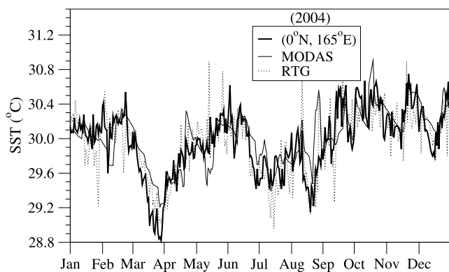
Figure 10. The same as Figure 8 but in 2004.
