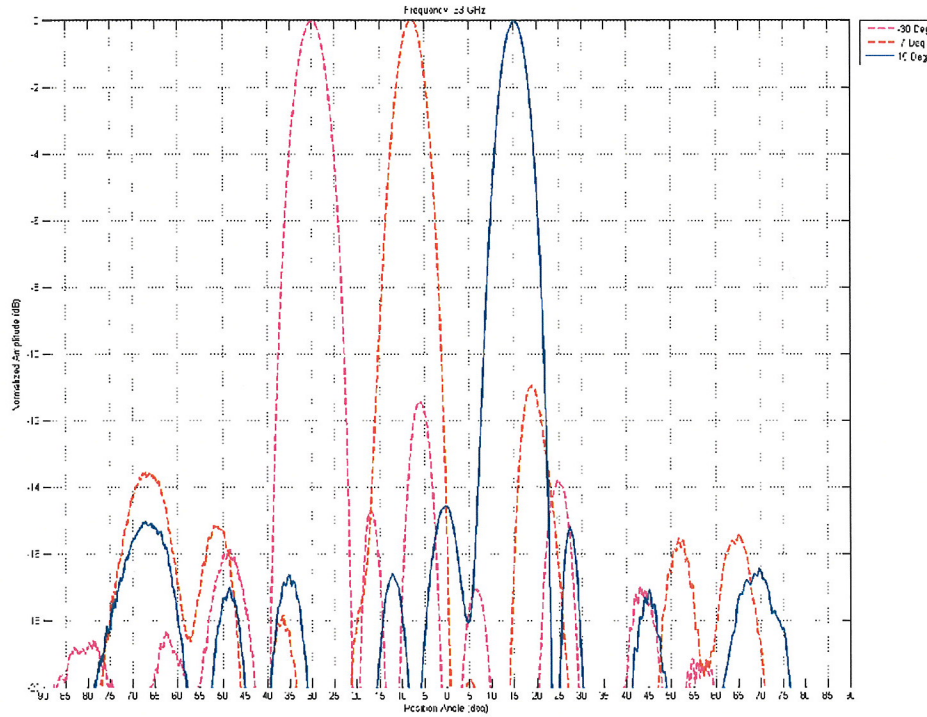
Figure 28. 33 GHz Pattern Measurements
