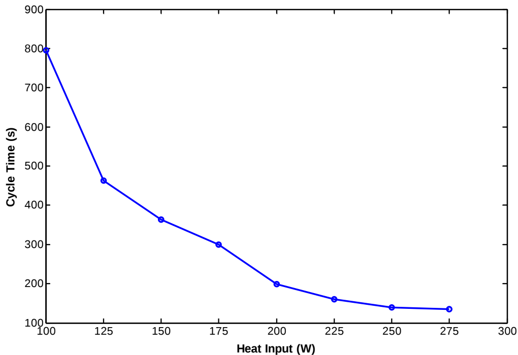
Figure 4.17: Effect of thermal load on the cycle time working with water for E75C50
