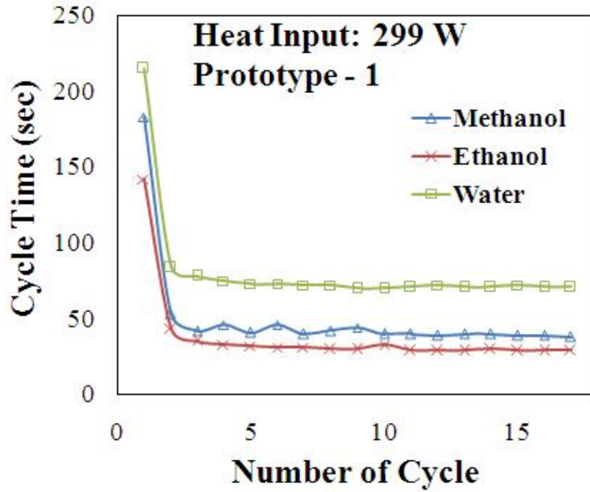
Figure 4.18: Effect of working fluids on cycle time during operation for thermolooop E75C50
