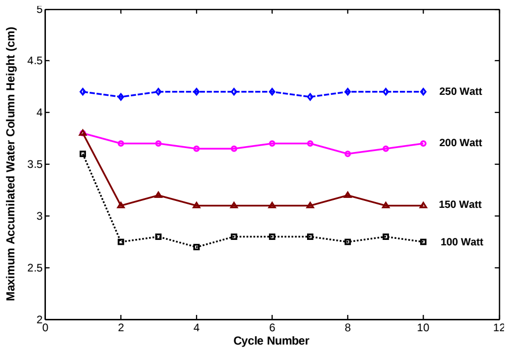
Figure 4.14: Variation of maximum system pressure during operation of the thermoloop device (E75C50) working with water for different heat loads
