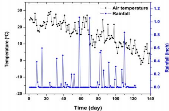
The air temperature and precipitation data of July 1 st to November 30 th , 2007.
