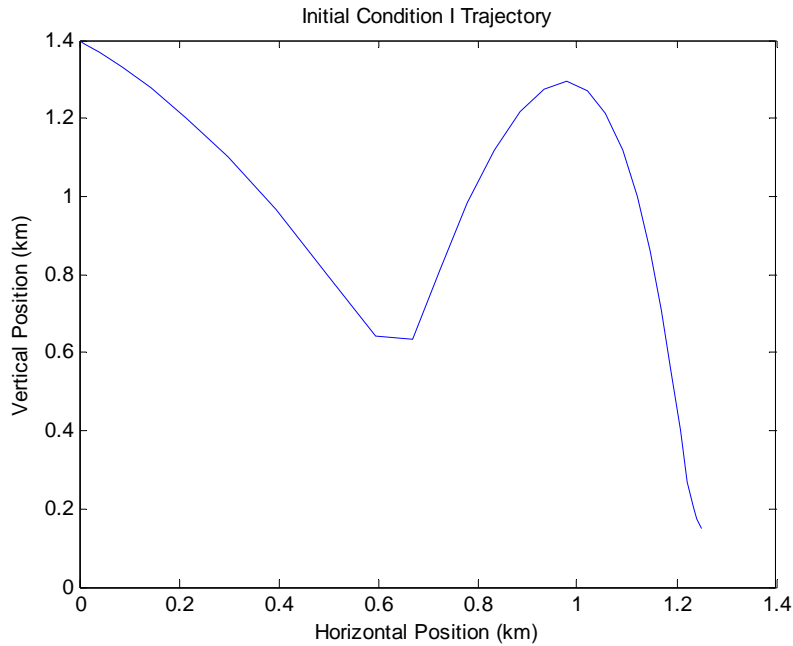
Figure 10. Initial Condition I – Trajectory
