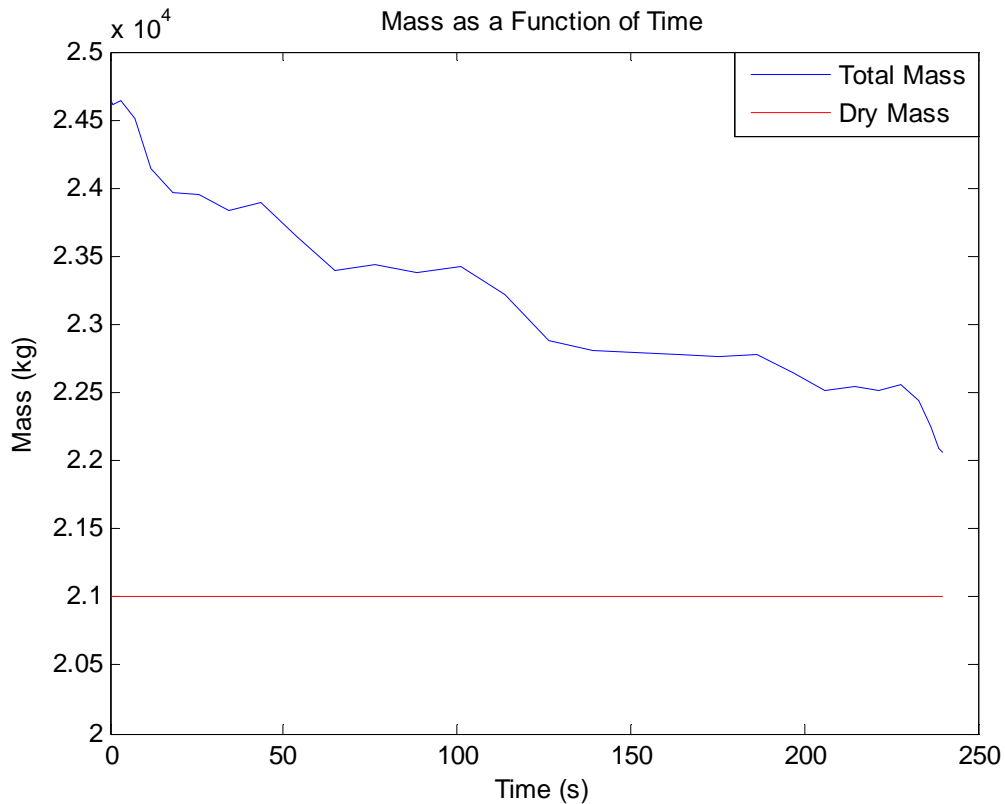
Figure 17. Initial Condition II – Mass
