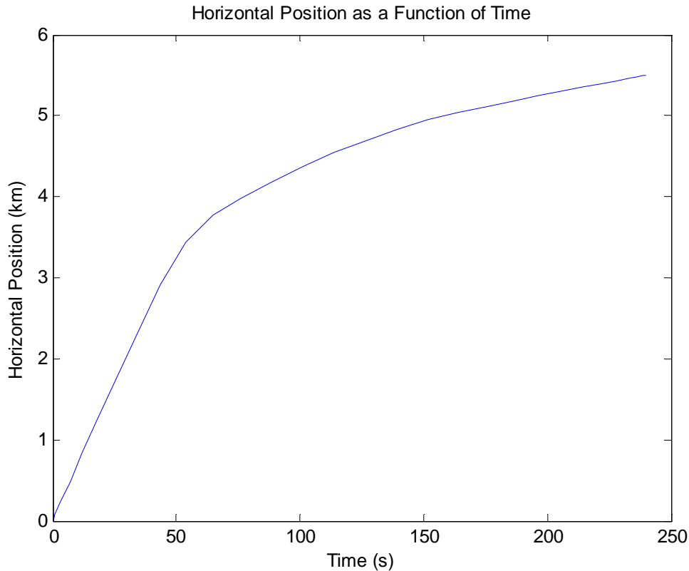
Figure 16. Initial Condition II – Horizontal Position
