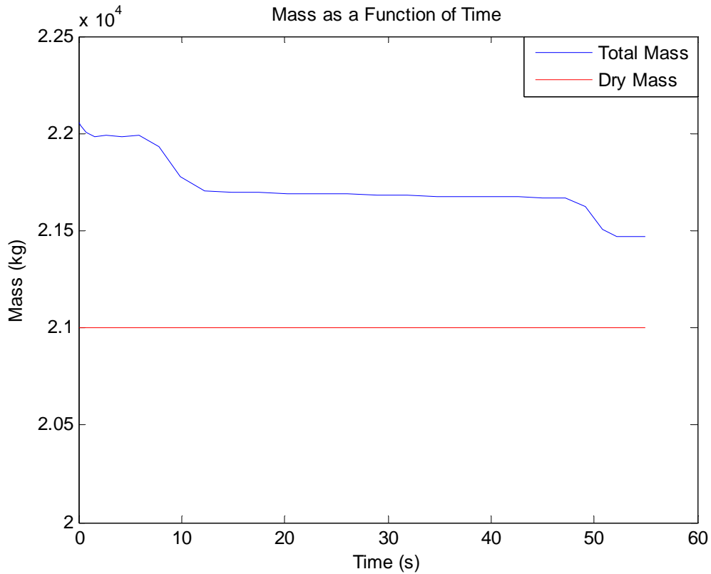
Figure 21. Redesignation Point – Mass
