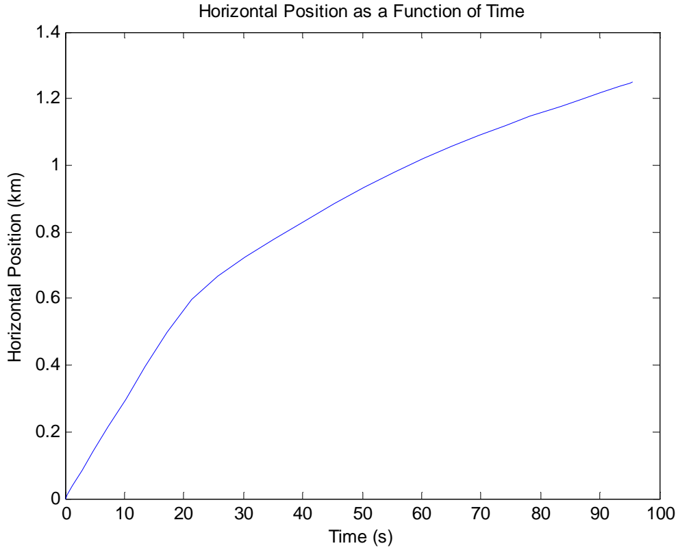
Figure 12. Initial Condition I – Horizontal Position
