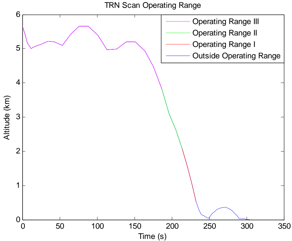
Figure 36. Initial Condition II – TRN Scan Range
