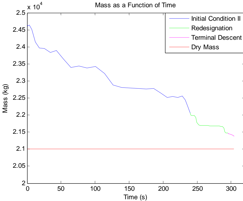
Figure 33. Complete Initial Condition II Trajectory – Mass
