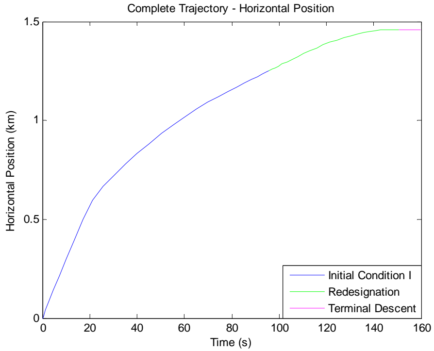
Figure 30. Complete Initial Condition I Trajectory – Horizontal Position
