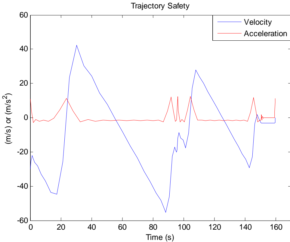
Figure 38. Initial Condition I Trajectory – Safety
