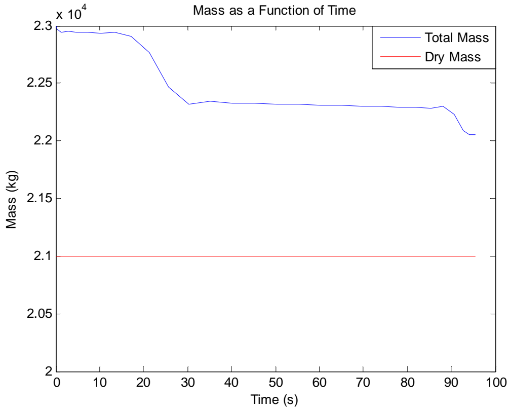
Figure 13. Initial Condition I – Mass
