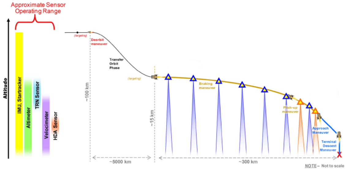
Figure 6. Sensor Operational Ranges 15
