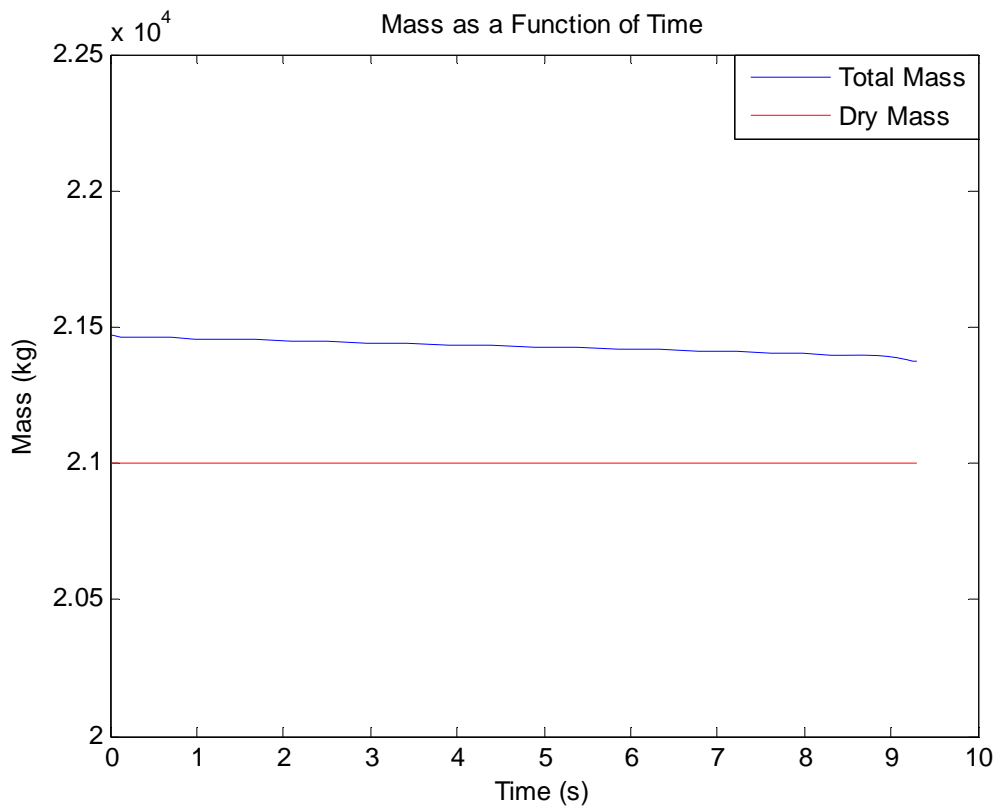
Figure 25. Terminal Descent – Mass
