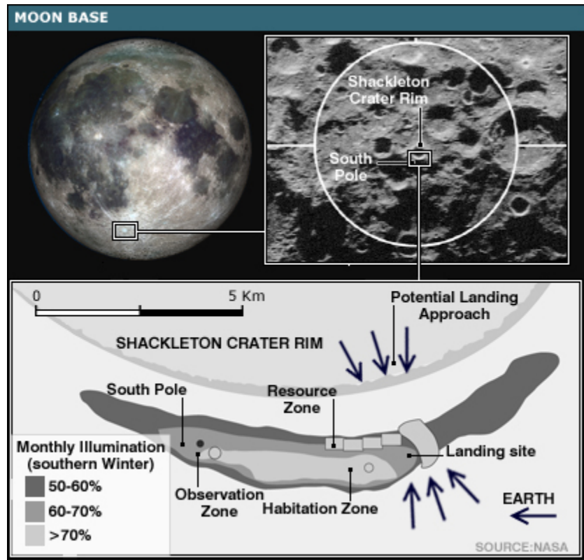
Figure 4. Proposed Shackleton Crater Outpost
