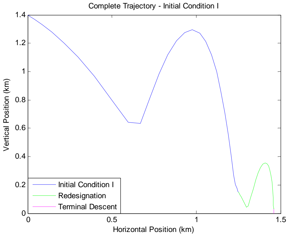
Figure 26. Complete Initial Condition I Trajectory
