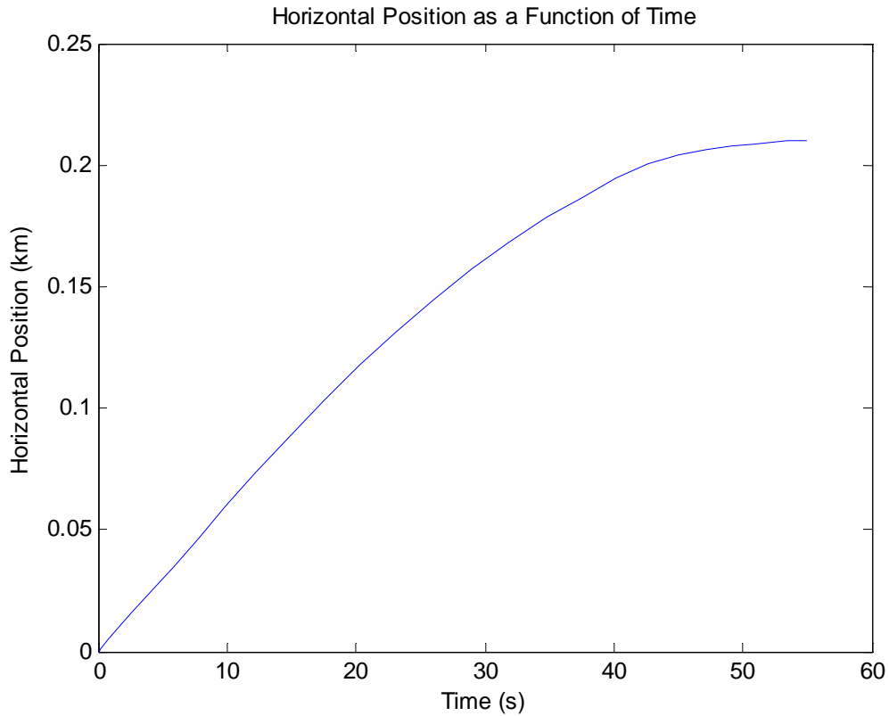
Figure 20. Redesignation Point – Horizontal Position
