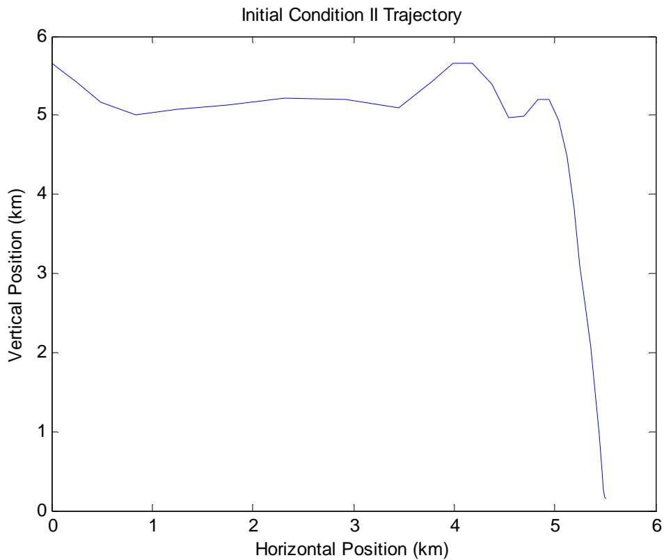
Figure 14. Initial Condition II – Trajectory
