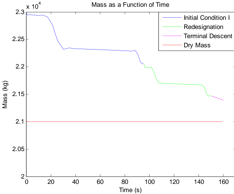
Figure 32. Complete Initial Condition I Trajectory – Mass
