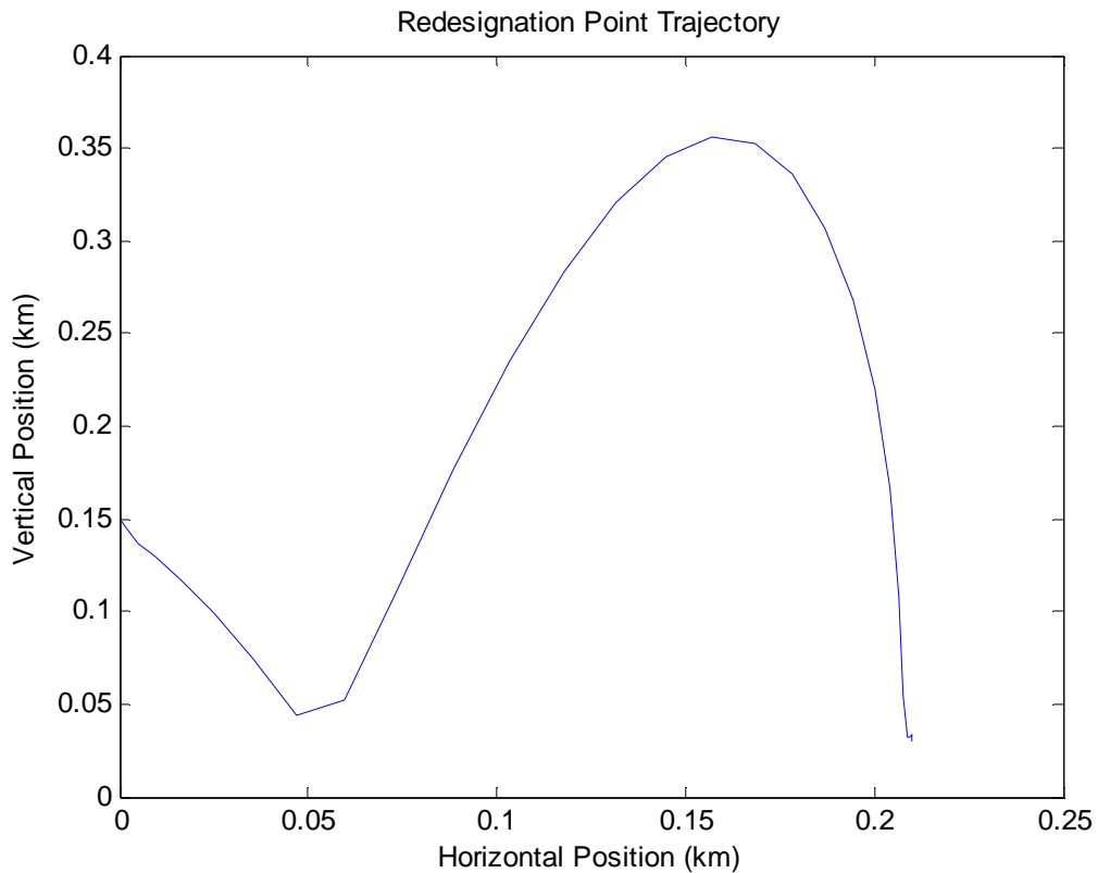
Figure 18. Redesignation Point – Trajectory
