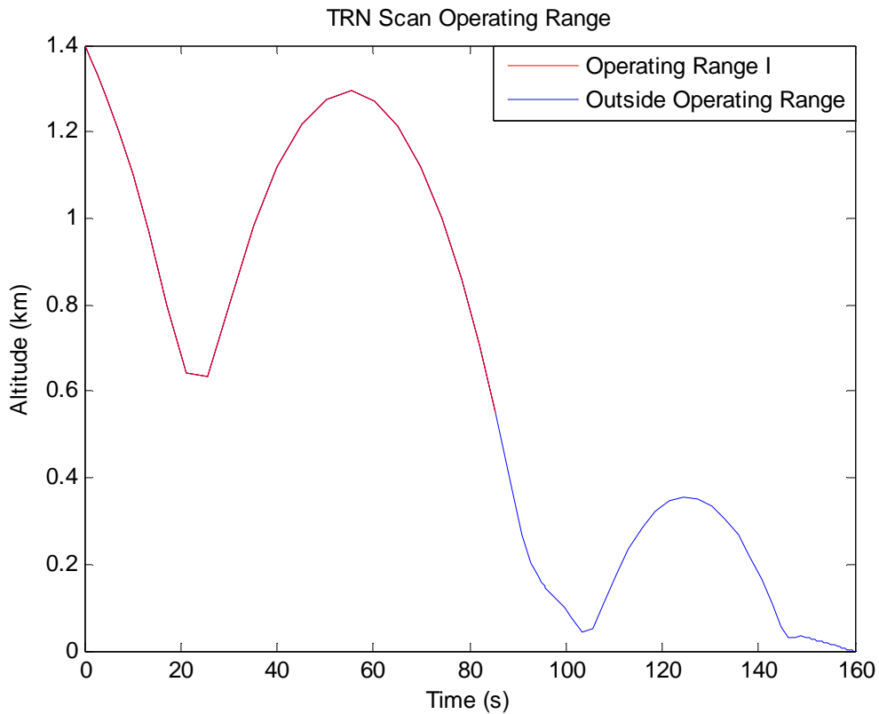
Figure 35. Initial Condition I – TRN Scan Range
