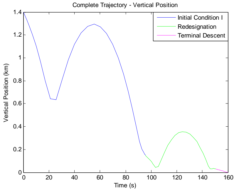
Figure 28. Complete Initial Condition I Trajectory – Vertical Position
