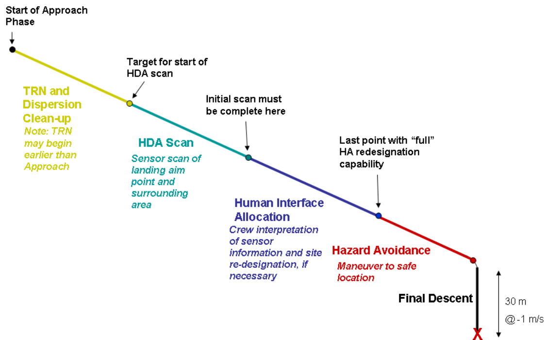
Figure 7. Approach Phase ConOps 18
