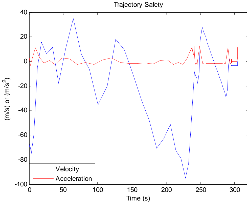
Figure 39. Initial Condition II Trajectory – Safety
