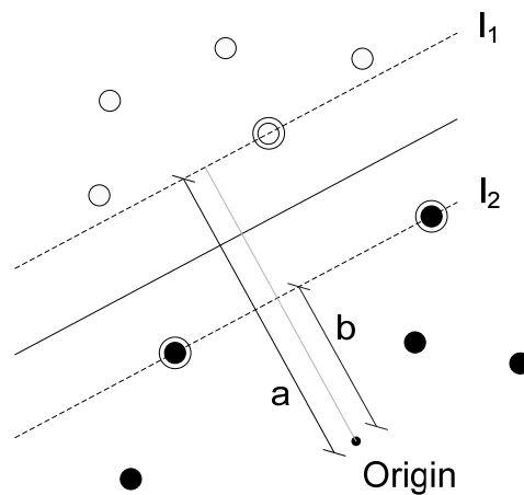
Figure 2. Linear Separating Hyperplanes [From 29].
