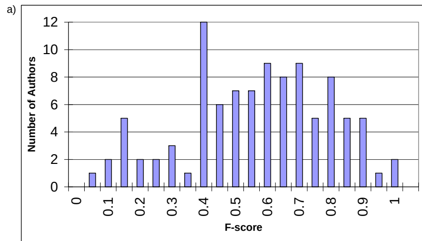
Figure 8. SVM: Data Set 3 (100 Authors): F-scores on Character 4-grams.
