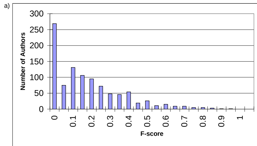
Figure 6. Naïve Bayes: Data Set 4 (1000 Authors): F-scores on Character Trigrams.
