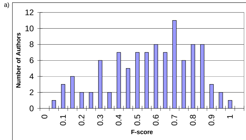
Figure 7. SVM: Data Set 3 (100 Authors): F-scores on Character Trigrams.
