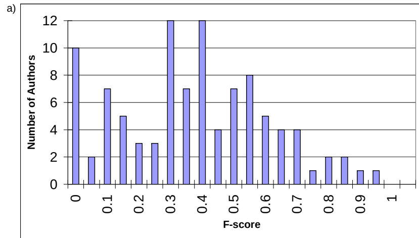
Figure 5. Naïve Bayes: Data Set 3 (100 Authors): F-scores on Character Trigrams.
