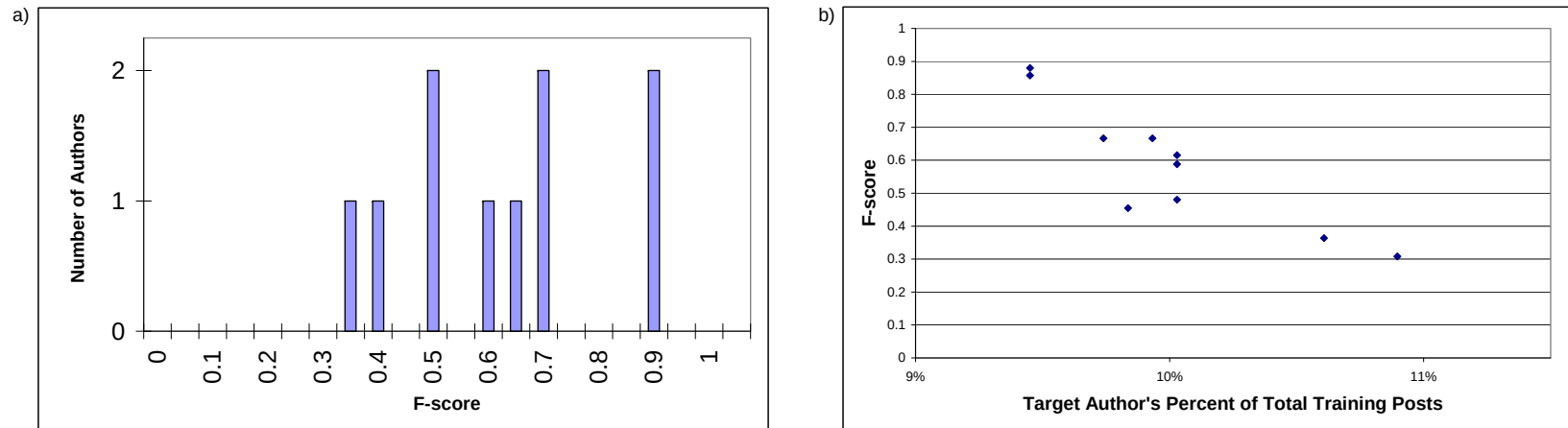
Figure 3. Naïve Bayes: Data Set 1 (10 Authors): F-scores on Character Bigrams.
