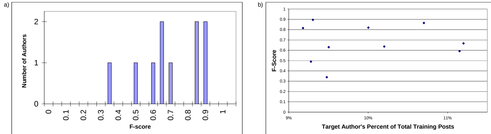
Figure 4. Naïve Bayes: Data Set 2 (10 Authors): F-scores on Character Trigrams.
