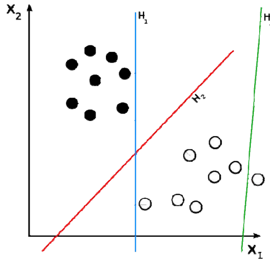
Figure 1. Linear Classification [From 31].
