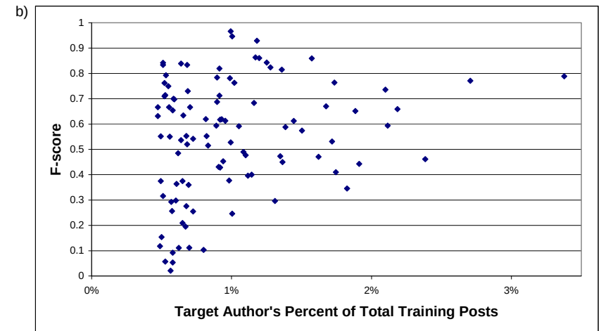
Figure 7. SVM: Data Set 3 (100 Authors): F-scores on Character Trigrams.
