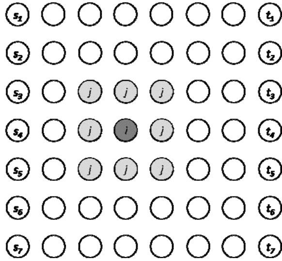
Figure 2. Network topology used by Bekker and Schmid (2006). They use a regular, square grid of nodes and connect each node i to each of its nearest neighbors j , using a directed arc (i, j) . Note that “nearest neighbors” includes nodes that are diagonally adjacent. For simplicity, no arcs are shown.
