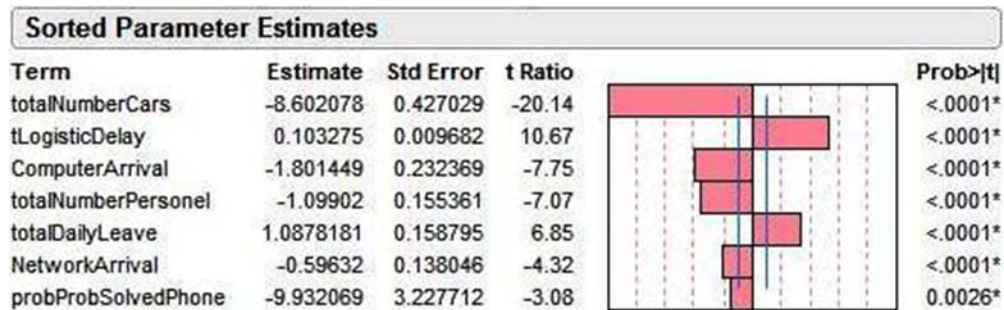
Figure 22. Sorted parameters for mean time in system
