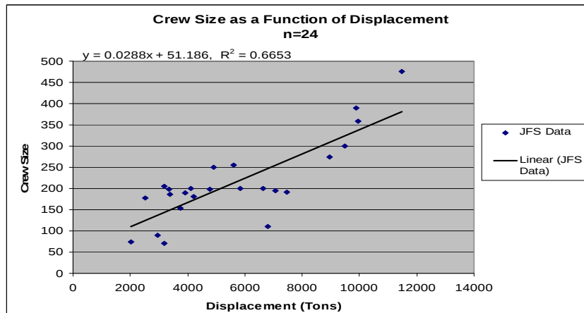
Figure 17. NGFS Crew Size as a Function of Tonnage
