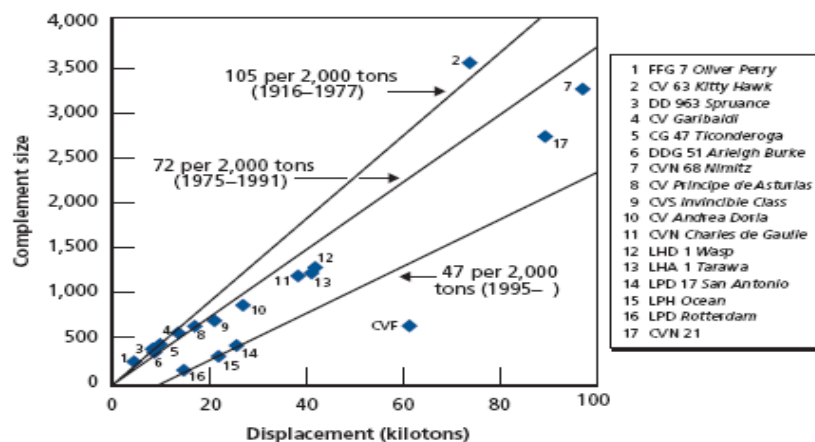
Figure 5. Technology Effects on Manpower Needs (From Schank et al., 2005, p. 71)
