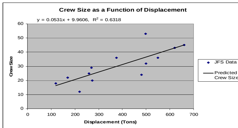
Figure 22. CC Crew Size as a Function of Tonnage
