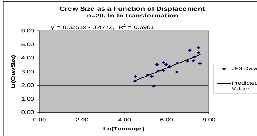
Figure 21. OPC Crew Size as a Function of Tonnage, ln-ln Transformation
