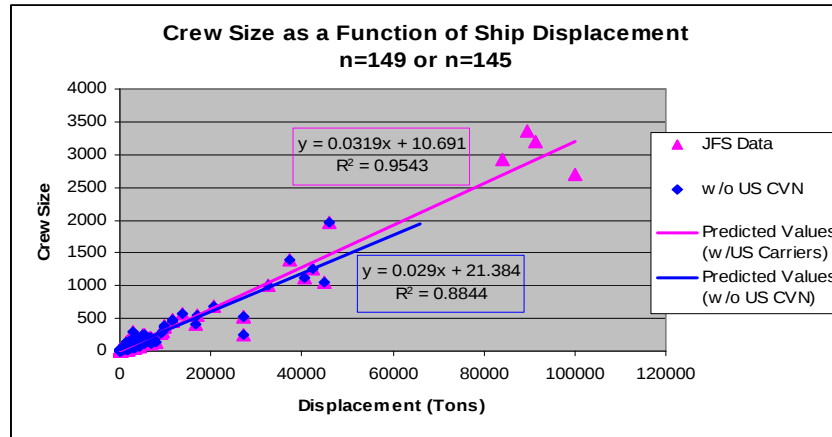
Figure 6. Warship Crew Sizes as a Function of Tonnage
