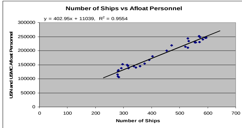
Figure 4. Afloat Personnel versus Number of Ships
