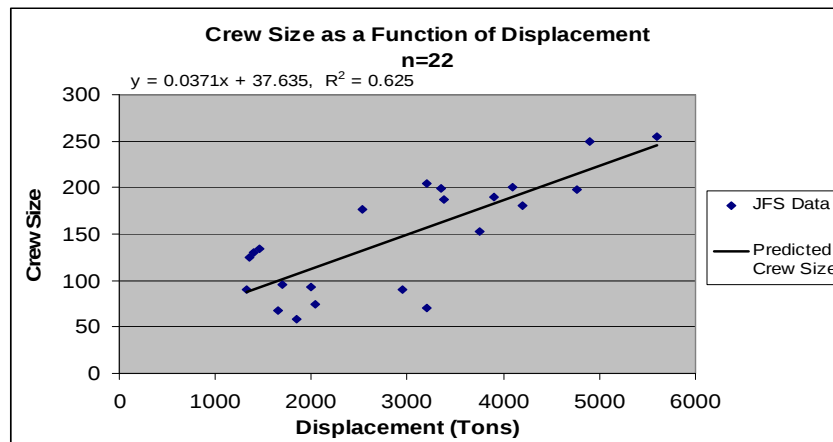
Figure 15. Frigate Crew Size as a Function of Tonnage
