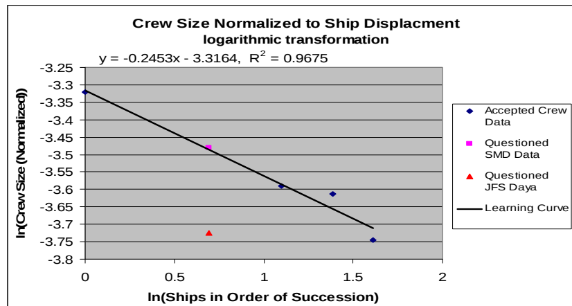
Figure 9. Logarithmic Transformation of Crew Size
