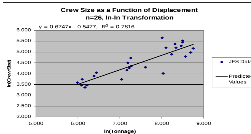
Figure 19. ASW Ship Crew Size as a Function of Tonnage, In-In Transformation
