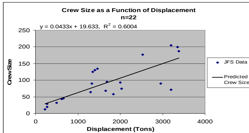
Figure 16. Land Attack Crew Size as a Function of Tonnage
