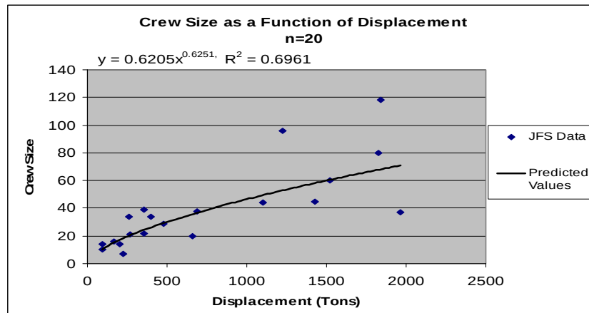
Figure 20. Offshore Patrol Craft Crew Size as a Function of Tonnage
