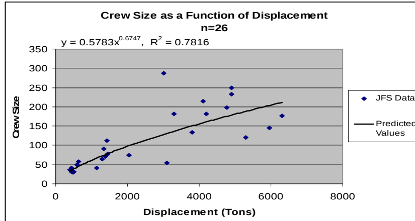
Figure 18. ASW Ship Crew Size as a Function of Tonnage
