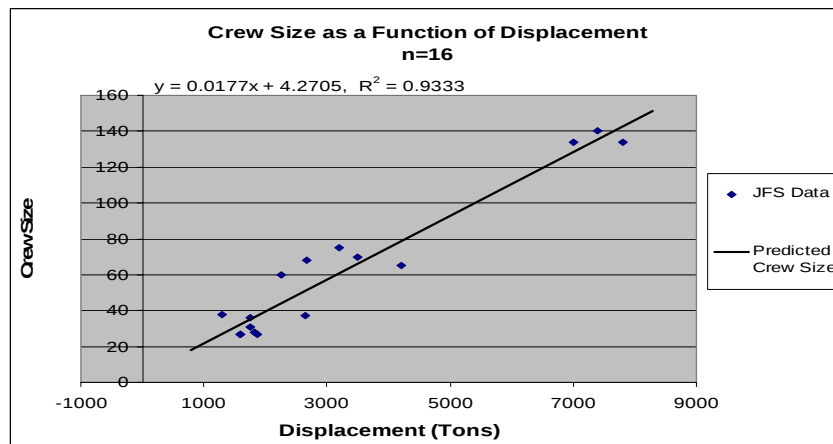
Figure 23. AIP submarine Crew Size as a Function of Tonnage
