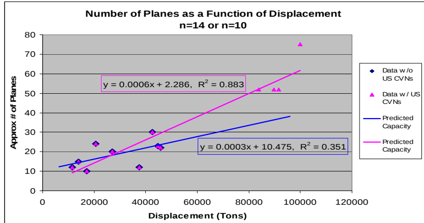
Figure 11. Number of Planes as a Function of Size
