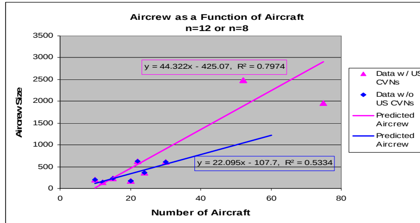
Figure 14. CV Aircrew Size as a Function of Aircraft (Alternate Analysis)
