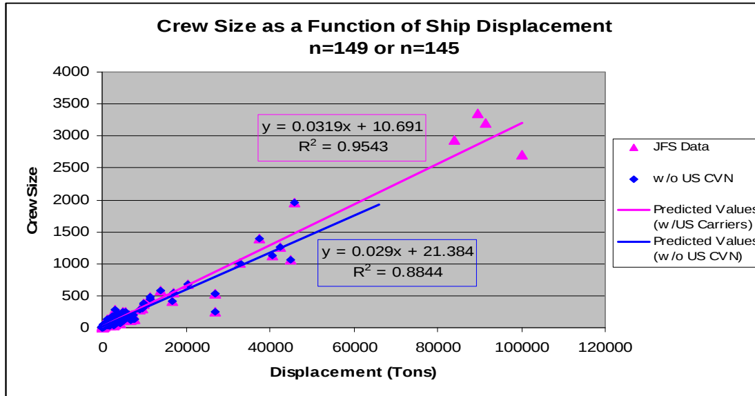
Crew Size as a Function of Displacement on Warships
