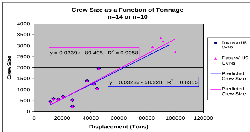
Figure 12. CV Crew Size as a Function of Tonnage
