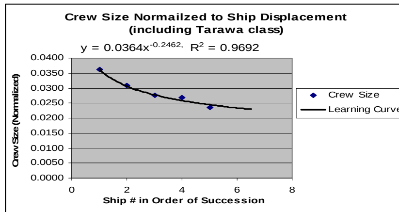
Figure 10. Normalized Crew Size
