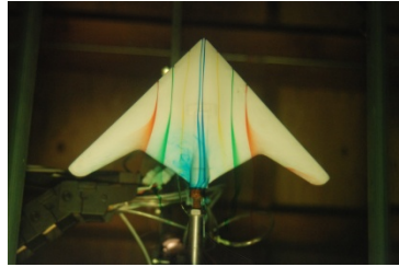
AoA, \alpha=4^\circ
