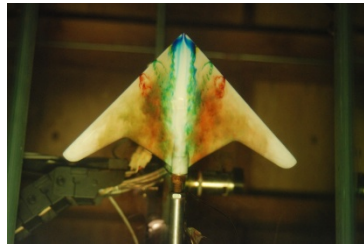
AoA, \alpha=20^\circ
