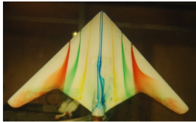
Re=2.15 \times 10^4
