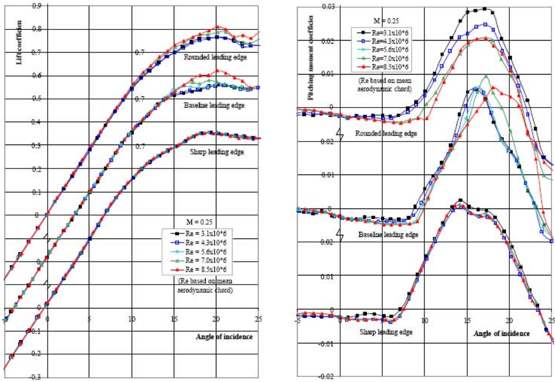
Figure 6 Variation of Lift Coefficient and Pitching Moment with Reynolds Number, From [4]
