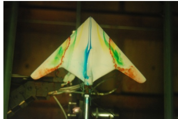
AoA, \alpha=10^\circ
