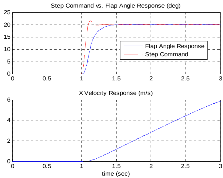
Figure 18. Longitudinal Flap Angle Response
