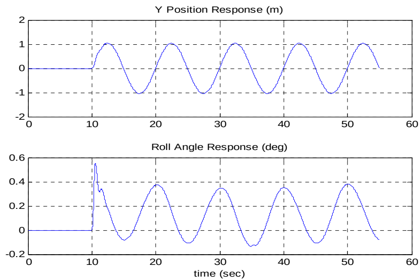
Figure 51. Roll Angle Response/Figure 9
