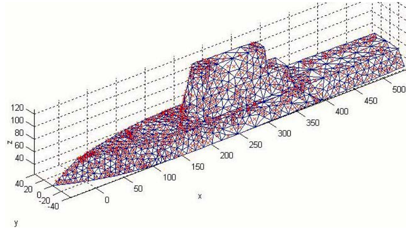
Figure 5. CAD model of DDG–1000 with 1200 distributed arrays (From [14])
