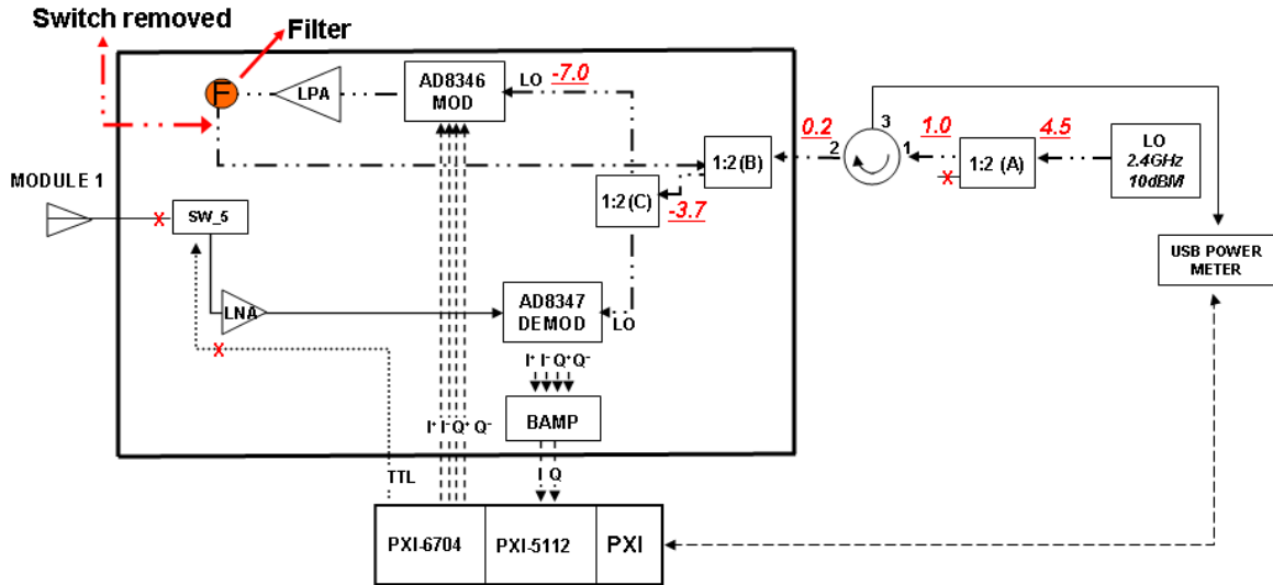
Figure 41. Measurement of LO signal power level in T/R module 1 with MFC-13944 and LPA implemented
