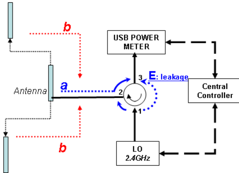
Figure 78. Two main factors affecting the leakage signal: (a) antenna mismatch and (b) reflection from outside environment
