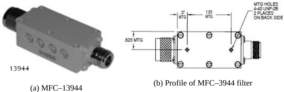
Figure 37. Model 13944 full band bandpass filter (From [44])
