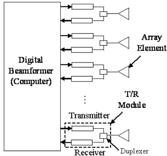
Figure 11. Generic DBF architecture (From [3])
