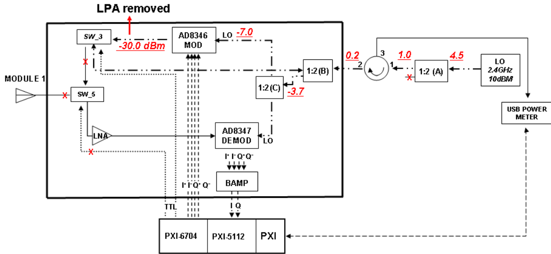
Figure 33. Measurement of LO signal power level in T/R module 1 without LPA (power in dBm)
