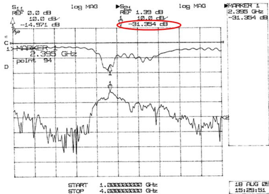
Figure 65. The system loss of two stubby antennas placed 50 cm apart
