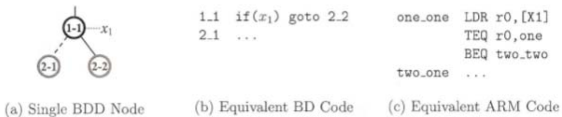
Figure 9. Comparison of BD Machine Code and Microprocessor Machine Code [15]
