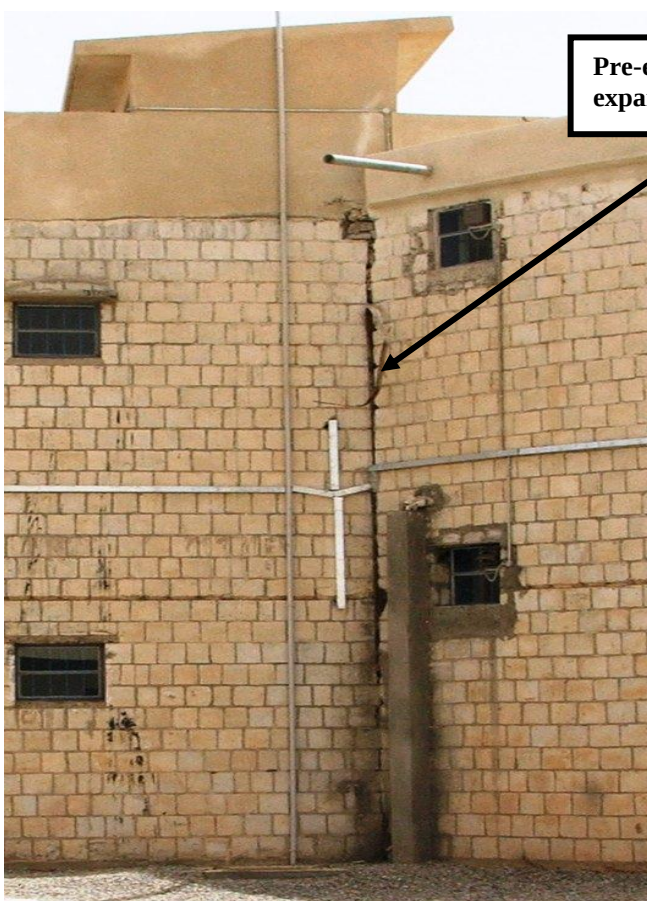
Site Photos 25 and 26. Pre-existing external expansion joints
