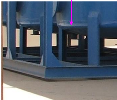
Site Photo 14. Equipment not bolted to slab.
