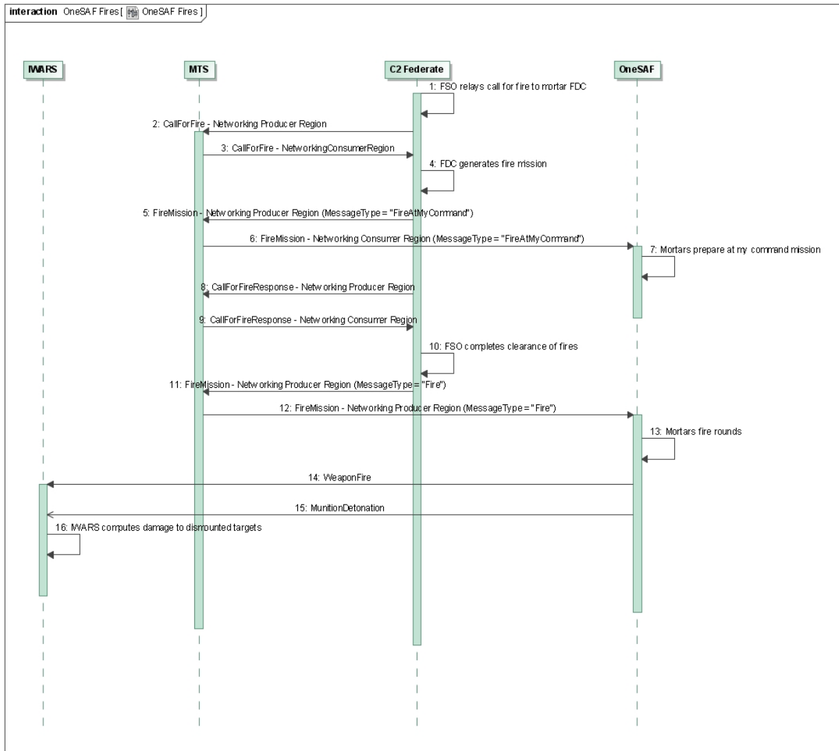
Figure 18: OneSAF fires sequence diagram. This diagram shows the sequence of messages required for OneSAF to fire mortar rounds in response to fire missions generated by the fires federate. The fires federate replicates the role of the fire direction center (FDC) that generates the fire mission and the fire support officer (FSO) who clears fires for the mission. First the FDC generates a fire mission in response to the call for fire message. The fire mission is passed via the MTS service to see if it can be delivered to the mortar unit. Once delivered, the mortars go through the process of laying the guns on the target and await a final fire message. In parallel with the process of laying the guns, the FSO conducts clearance of fires to ensure no friendly forces are in the vicinity of the mission. Once clearance of fires is complete, the FSO sends a fire message to the guns in order to execute the mission. The guns fire, and a munition detonation interaction is sent to IWARS so that damage can be calculated against dismounted targets in the area.
