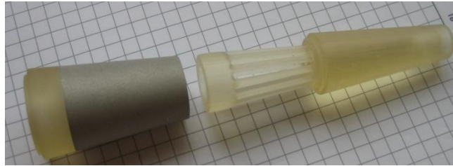
Figure 10. Porous injector.
