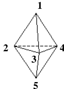
Figure 11. Example for which no more than N/2 matchings may be obtained.
