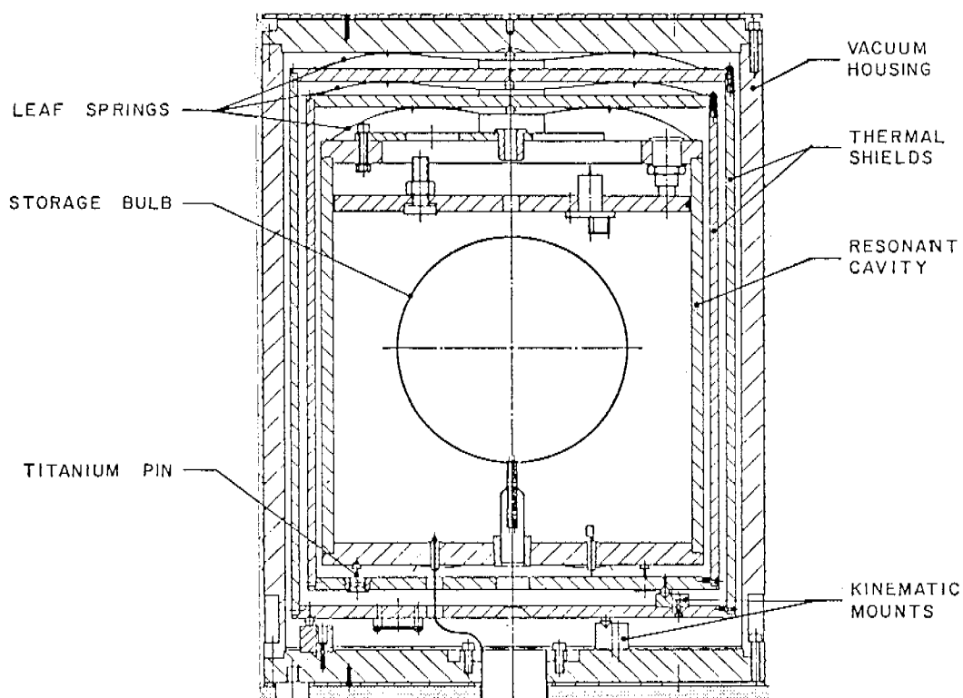
Fig. 2. Detail of cavity region showing thermal shields and kinematic supports.
