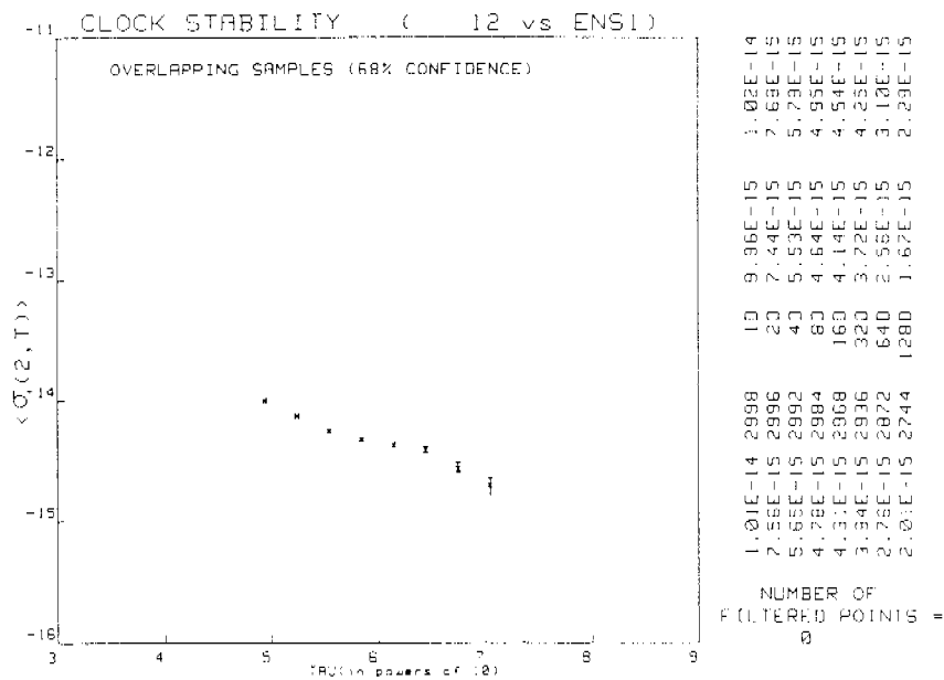
Figure 8: Output of algorithm using equal weights for all clocks (8 years of simulated data).
