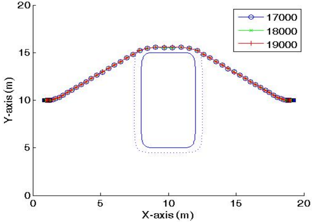
Figure 54. Solution Progression (17,000-19,000 Iterations).
