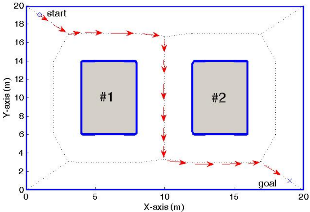
Figure 14. Voronoi Diagram for the Benchmark Case.
