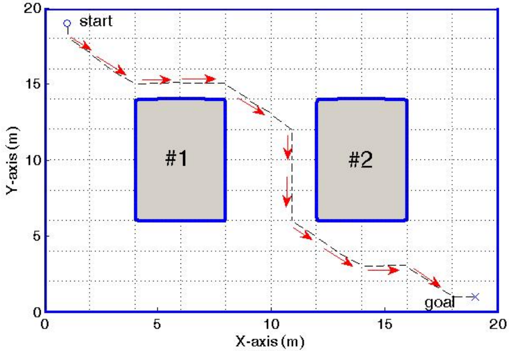
Figure 17. Fixed-size ACD for the Benchmark Case.
