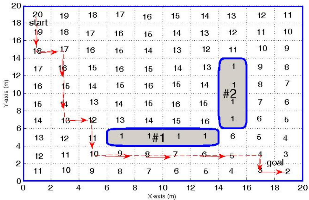
Figure 12. Wave-front Planner Overcomes Local Minimum Problem.
