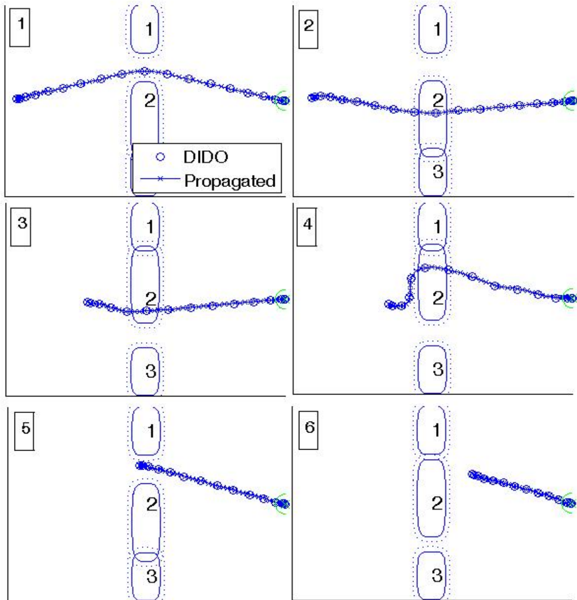
Figure 105b. Evolution of Cyclic Sliding Door (Prediction // 0.5 m/s cycle speed).
