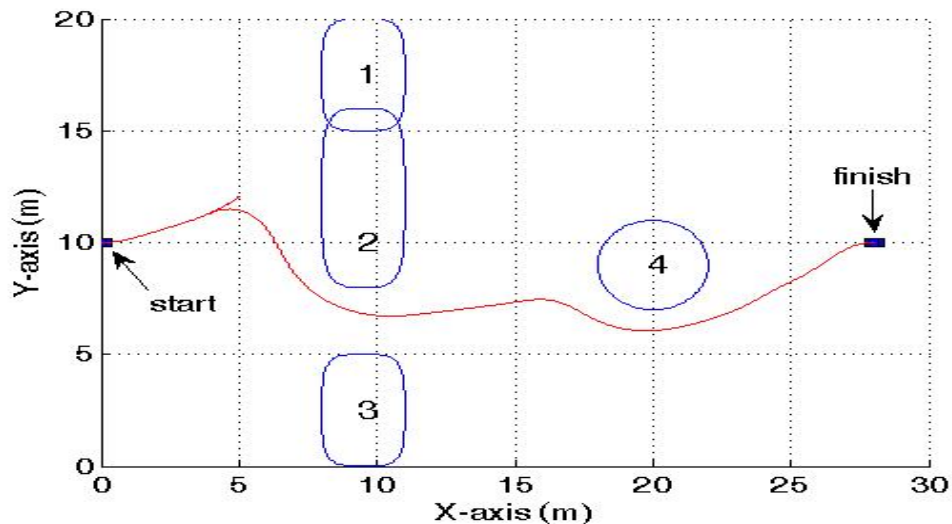
Figure 81. Vehicle Trajectory (Obstacle 4 Appears at t = 25 sec).
