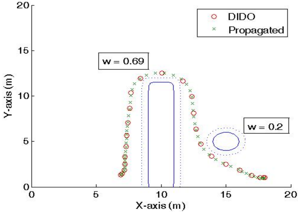
Figure 90. Vehicle Trajectory for a Two-obstacle Environment.
