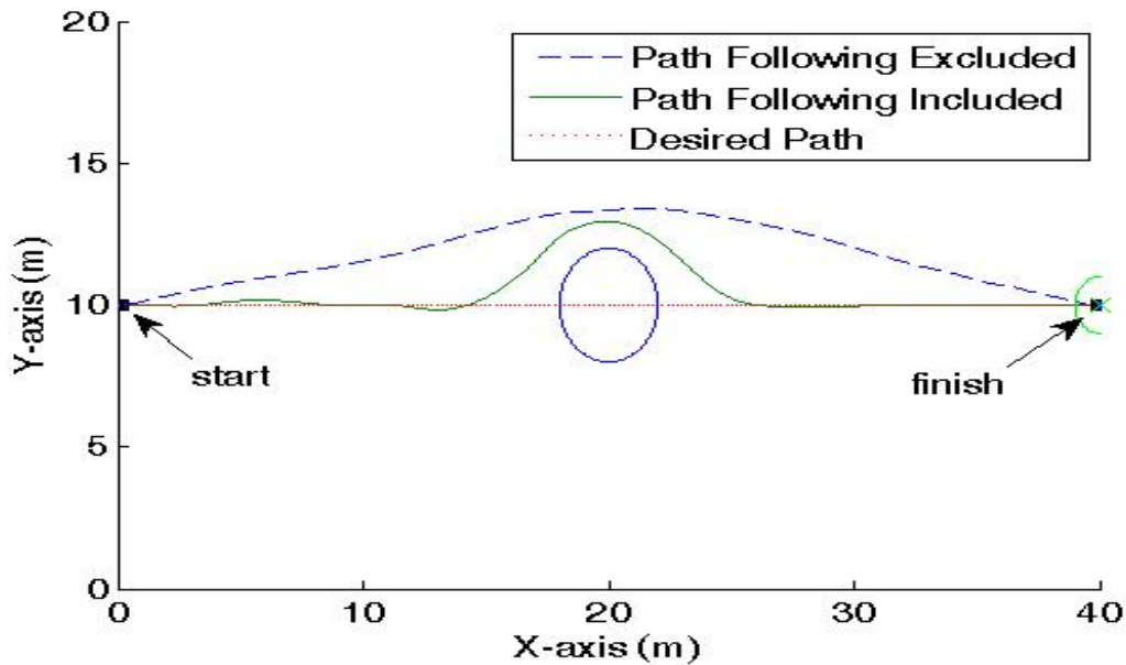
Figure 122. Path Following vs. Trajectory Planning with Known Obstacle.
