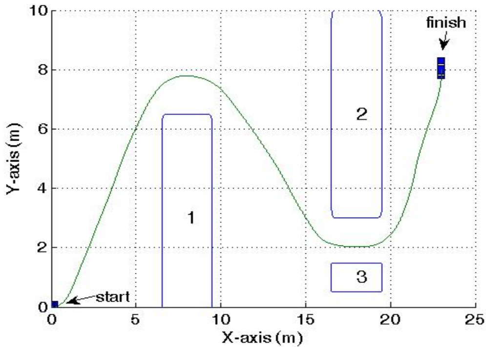
Figure 92. Vehicle Traversing a Narrow Passage.
