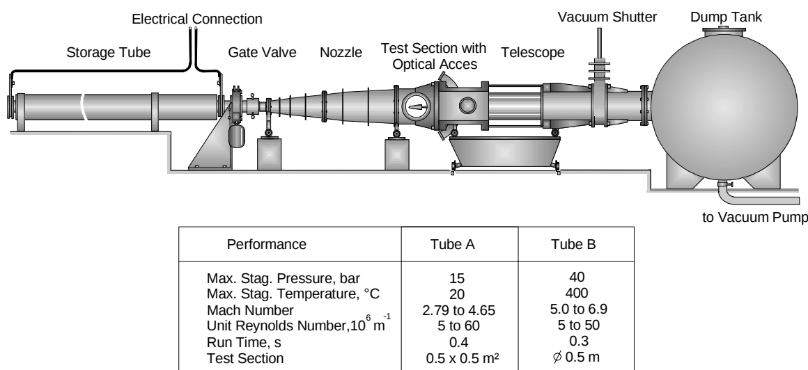
Figure 7: The RWG Ludwig Tube Facility in Göttingen.
