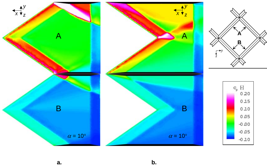
Figure 21: Surface pressure distribution on two typical members A and B of grid fins from valley-type LSLW v_10°_55°_0.714 (a) and from peak-type LSLW p_10°_55°_0.714 (b) at M_\infty = 4 and \alpha = 10^\circ .
