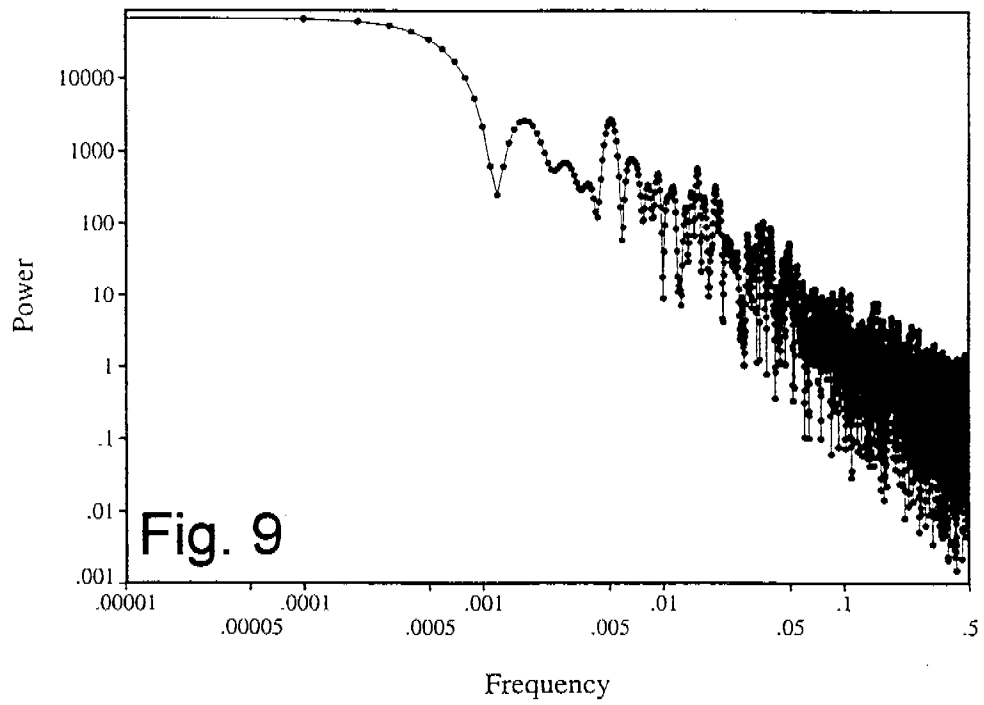
Power Spectral Density of White FM from the Digital-Spectrum-Analyzer Method
