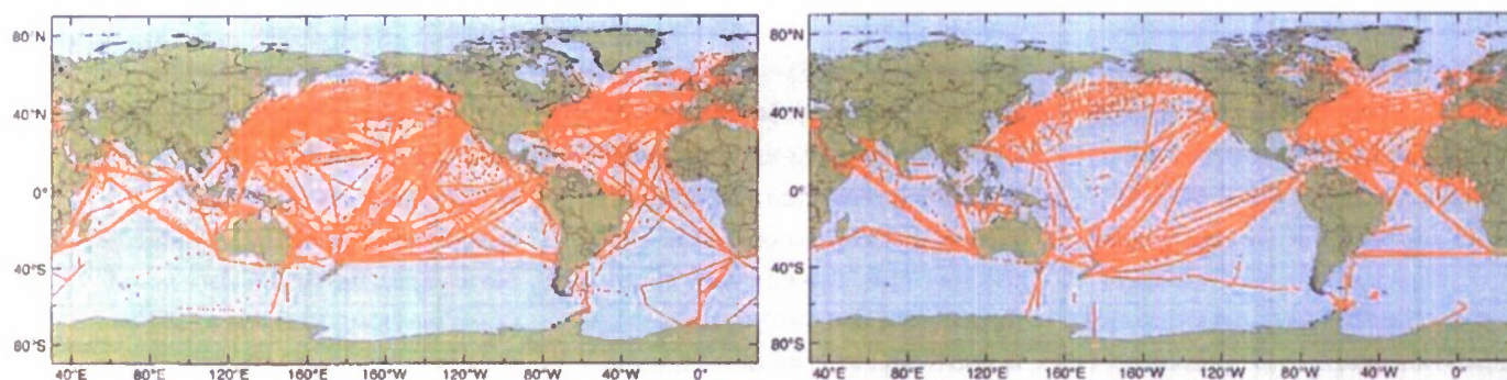
Figure 6. The global distribution of expendable bathythermograph (XBT) observations from ships of opportunity in 1999 (left) and 2005 (right). The total number of XBT profiles from the Ship of Opportunity Programme (SOOP) decreased during the GODAE period as the Argo array was implemented.
