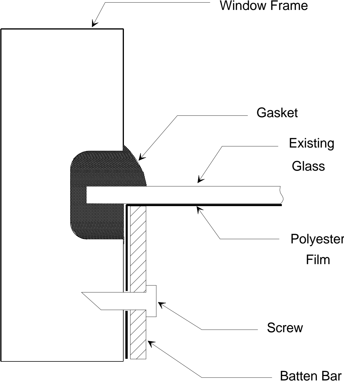
Figure 1. Anchored Film - Battened System
