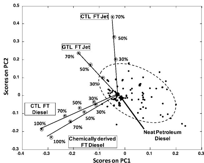
Figure 2. PCA scores plot showing how different synthetic fuels blended into F-76 naval distillate fuel can be discriminated.
