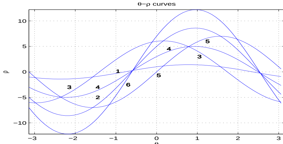
Figure 3. Transforms of M_n s in Figure 2 to \theta\rho p
