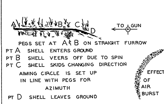
Figure 3a—Typical Ricochet Marks
