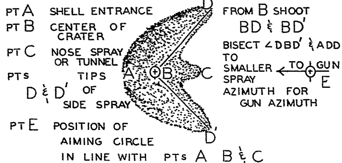
Figure 3b—Typical Shell Crater (FQ)
