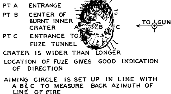
Figure 3c—Deep Shell Crater
