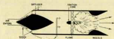
Figure 5. Ramjet engine.
