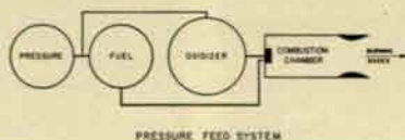
Figure 3. Liquid-propellant rocket.
