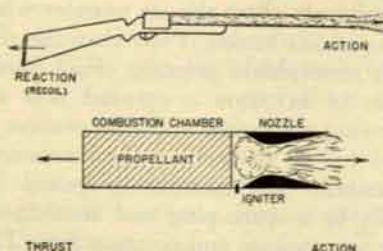
Figure 1. A rocket works like a shotgun.
