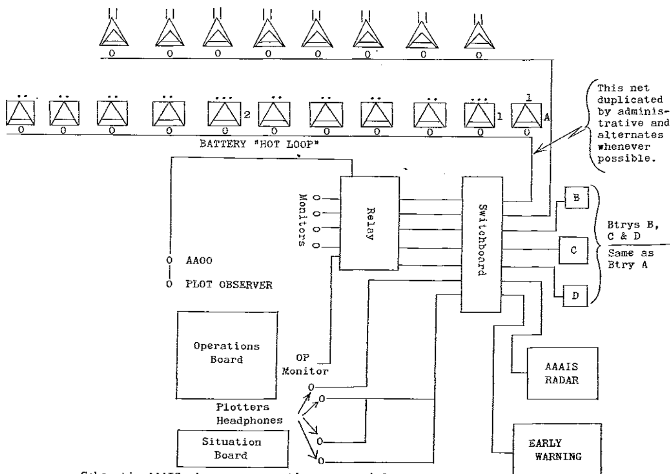
Schematic AAAIS wire net-automatic weapons defense
