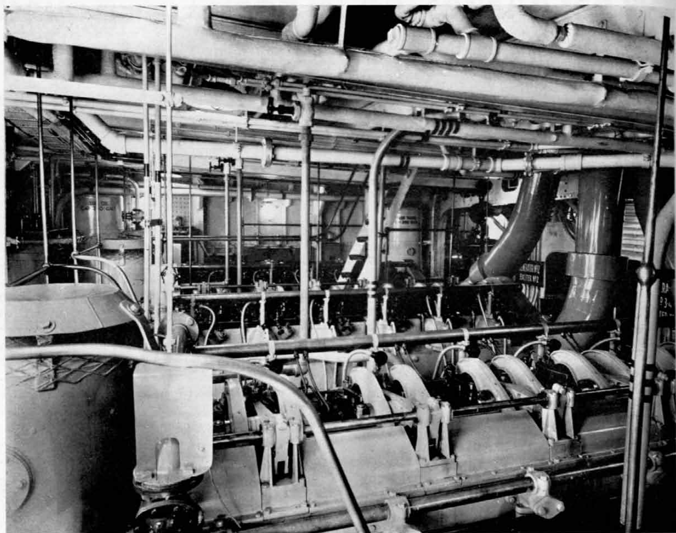
The engine room of the mine planter Ellery W. Niles. This vessel is powered by Diesel engines.
