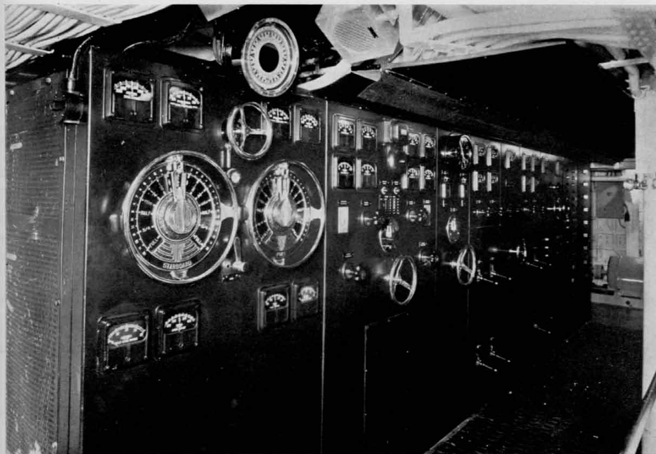
Switchboard of the engine room of the mine planter Ellery W. Niles .
